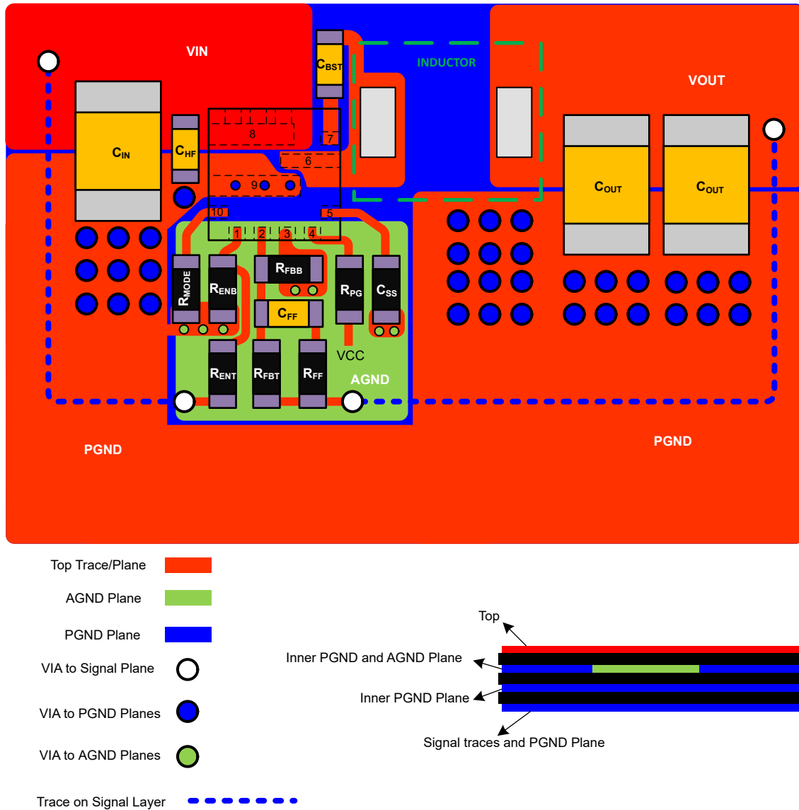
Figure 7-18. TPS56A37 layout
