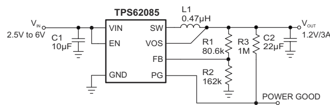
Figure 9-1. 1.2-V Output Voltage Application
