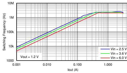
Figure 7-1. Switching Frequency
