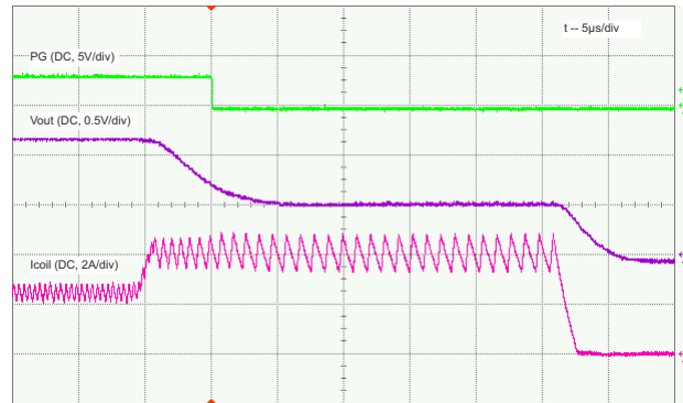
Figure 9-19. Output Short-Circuit Protection, Load = 0.47 \Omega , HICCUP Zoom In
