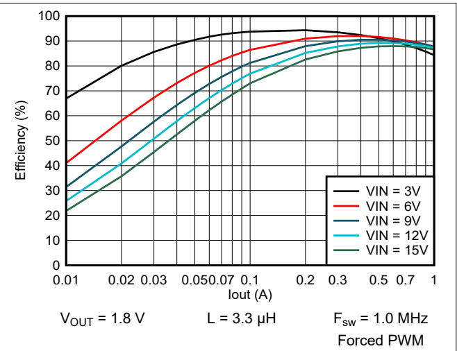
Figure 9-33. Efficiency vs Output Current
