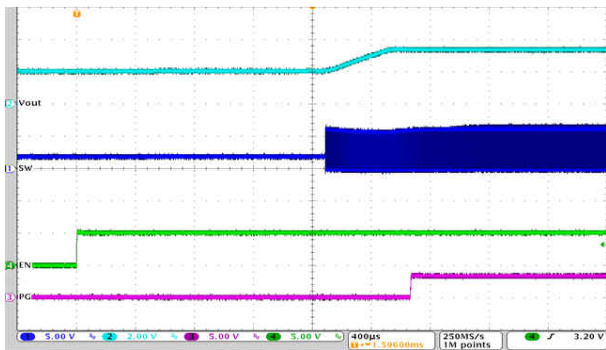
Figure 9-66. Start-Up Timing
