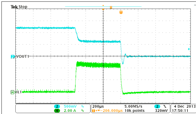
Figure 9-20. Buck1, OCP
