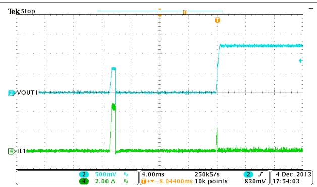
Figure 9-21. Buck1, Hiccup and Recovery
