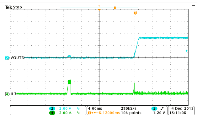
Figure 9-25. Buck3, Hiccup and Recovery
