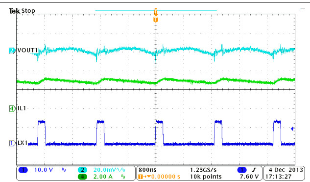
Figure 9-9. Buck1, Steady State Operation at Full Load
