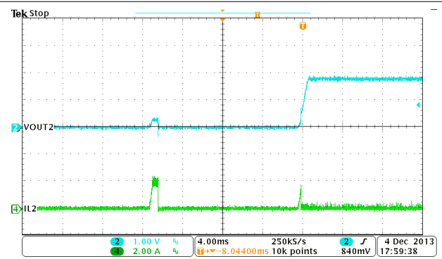
Figure 9-23. Buck2, Hiccup and Recovery
