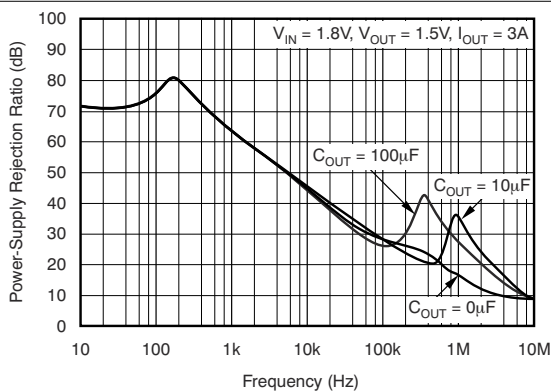
Figure 5-15. V_{IN} PSRR vs Frequency
