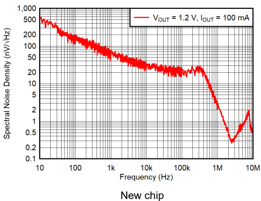
Figure 5-23. Noise Spectral Density
