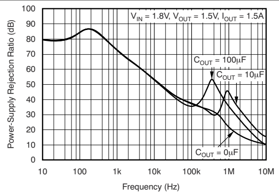
New chip Figure 5-14. V_{BIAS} PSRR vs Frequency
