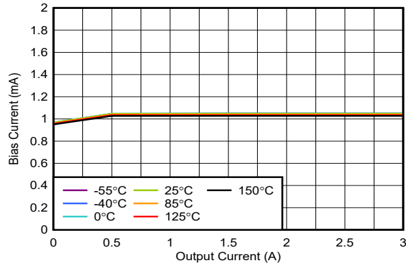
New chip, V_{IN} = 1.1\text{V} , V_{OUT} = 0.8\text{V}
