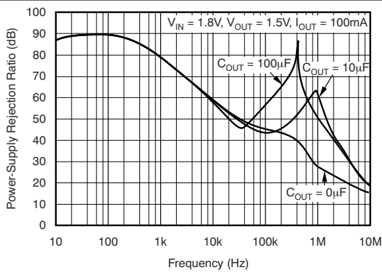
Legacy chip Figure 5-13. V_{BIAS} PSRR vs Frequency
