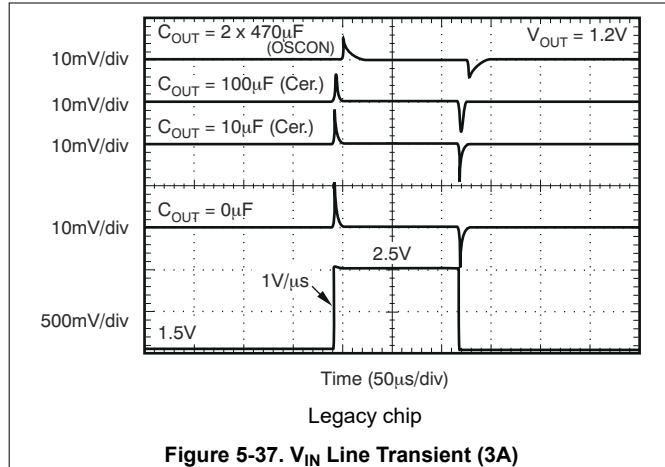
Figure 5-37. V_{IN} Line Transient (3A)
