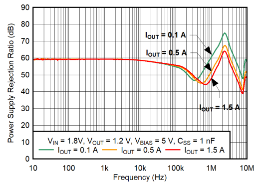
New chip Figure 5-14. V_{BIAS} PSRR vs Frequency
