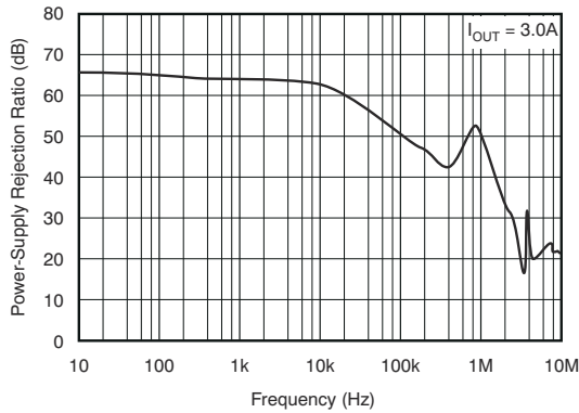
Legacy chip Figure 5-13. V_{BIAS} PSRR vs Frequency
