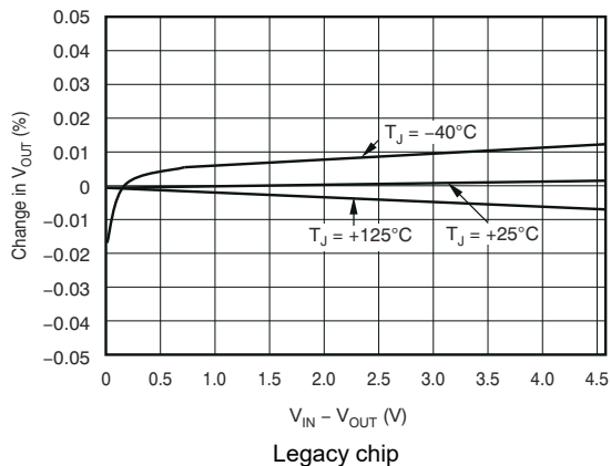
Figure 5-5. Line Regulation
