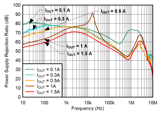
New chip Figure 5-18. V_{IN} PSRR vs Frequency
