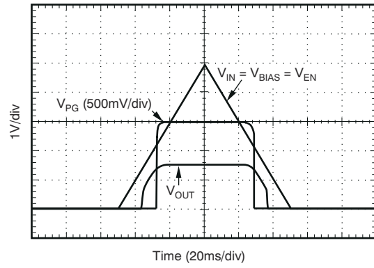
Figure 7-3. Power-Up, Power-Down
