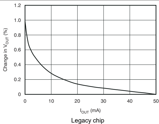
Legacy chip Figure 5-5. Load Regulation at Light Load
