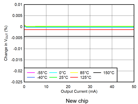
New chip Figure 5-6. Load Regulation at Light Load
