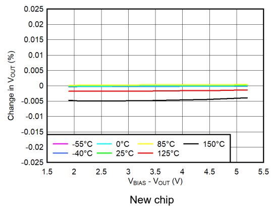
New chip Figure 5-4. V BIAS Line Regulation
