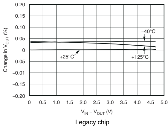
Legacy chip Figure 5-1. V IN Line Regulation
