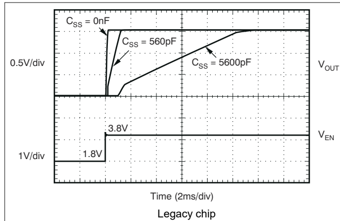
Figure 5-36. Turn-On Response
