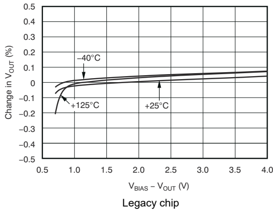
Legacy chip Figure 5-3. V BIAS Line Regulation
