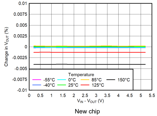
New chip Figure 5-2. V IN Line Regulation
