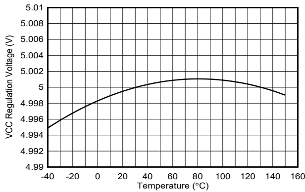
Figure 6-1. VCC Regulation Voltage vs Temperature
