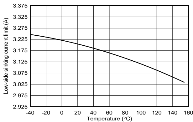
Figure 6-5. Low-Side Sinking Current Limit vs Temperature
