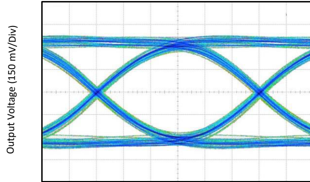
Figure 5-13. DisplayPort HBR3 Eye-Pattern Performance with 12-Inch Input PCB Trace at 8.1Gbps
