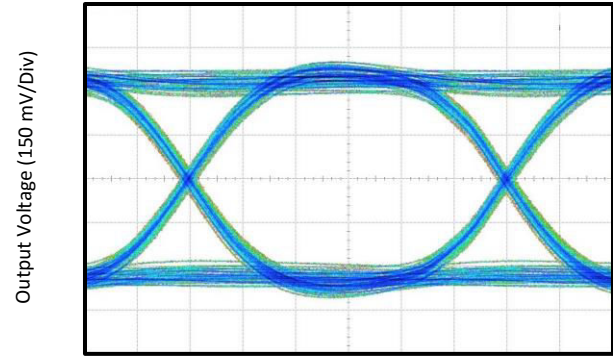
Figure 5-14. USB 3.1 Gen1 Eye-Pattern Performance with 12-Inch Input PCB Trace at 5Gbps
