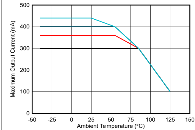
Figure 6-3. Maximum Output Current vs Ambient Temperature : VCC = 5.0V , C OUT2 = 22µF
