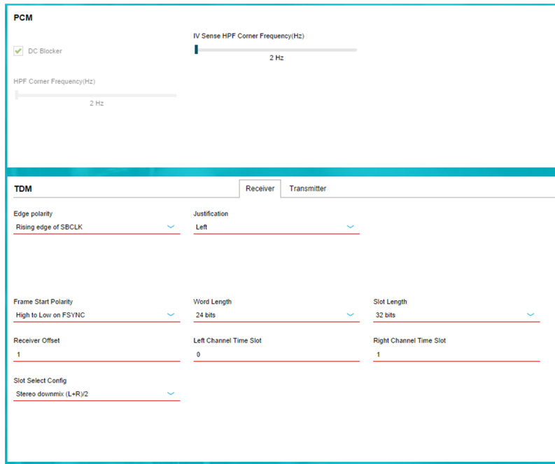
Figure 1-8. PCM and TDM Settings (Advance)
