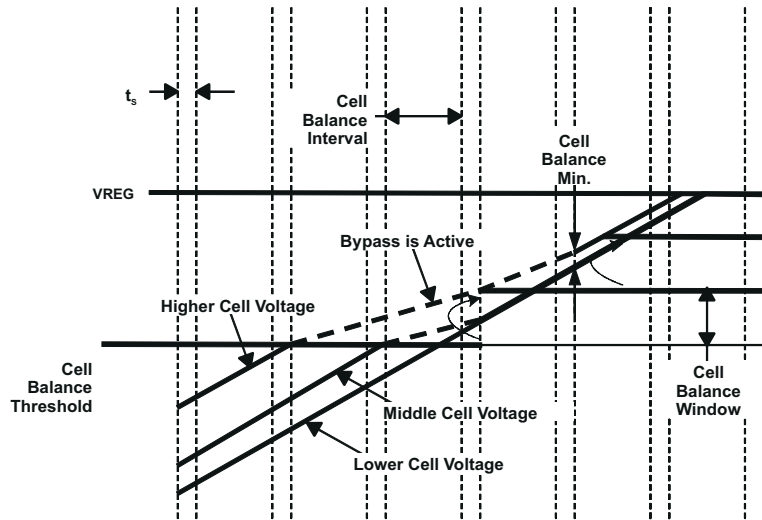
Figure 7-7. Cell Balancing
