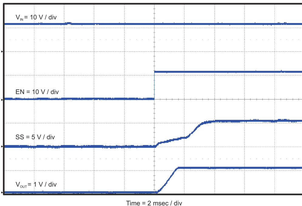
Figure 4-10. TPS54339EVM-056 Start-Up Relative to EN with SS
