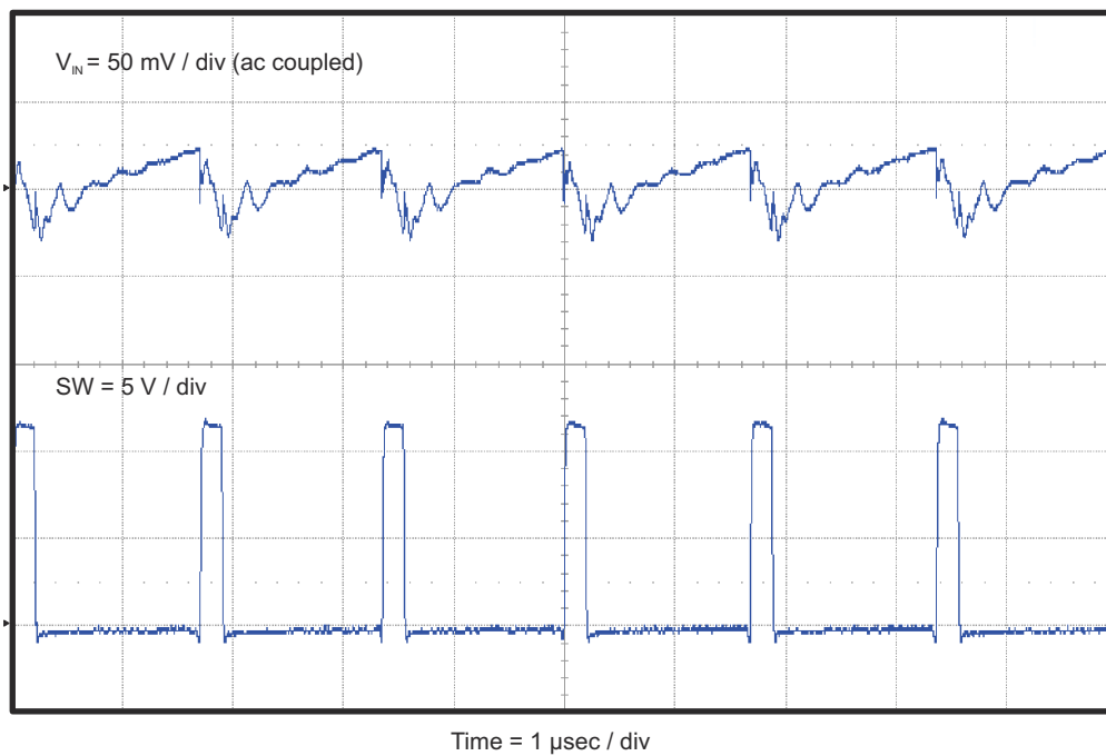
Figure 4-8. TPS54339EVM-056 Input Voltage Ripple
