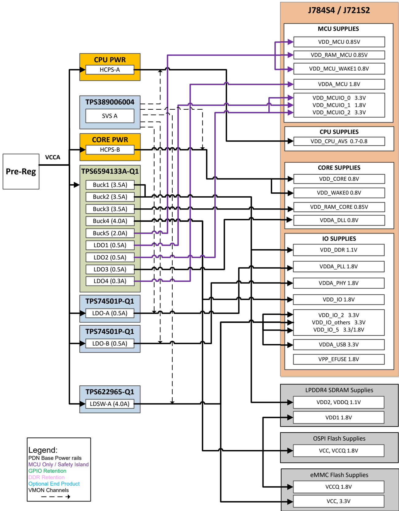
Figure 2-2. PDN-3F Power Connections - Reduced Features
