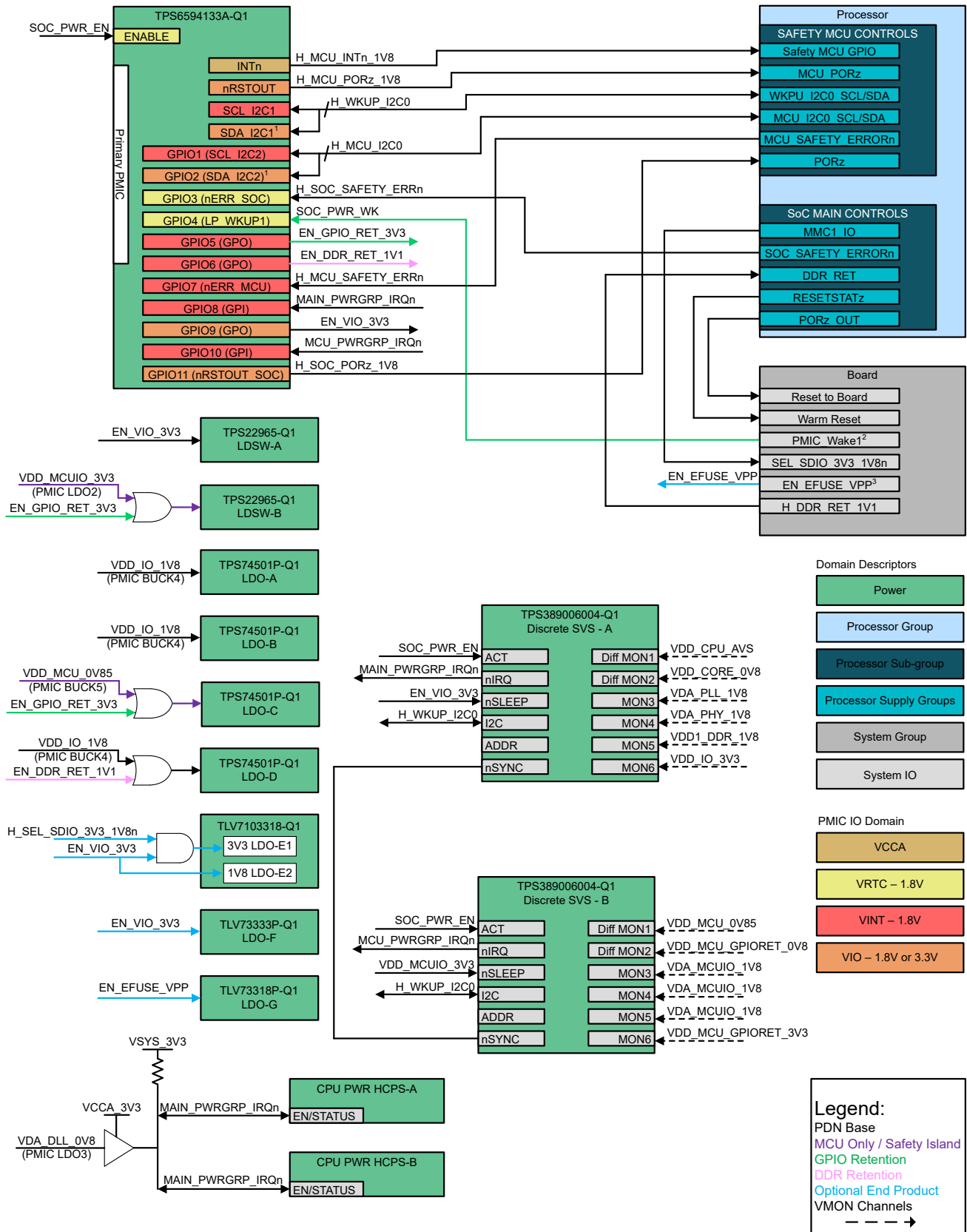
Figure 2-3. TPS6594133A Digital Connections for PDN-3A
