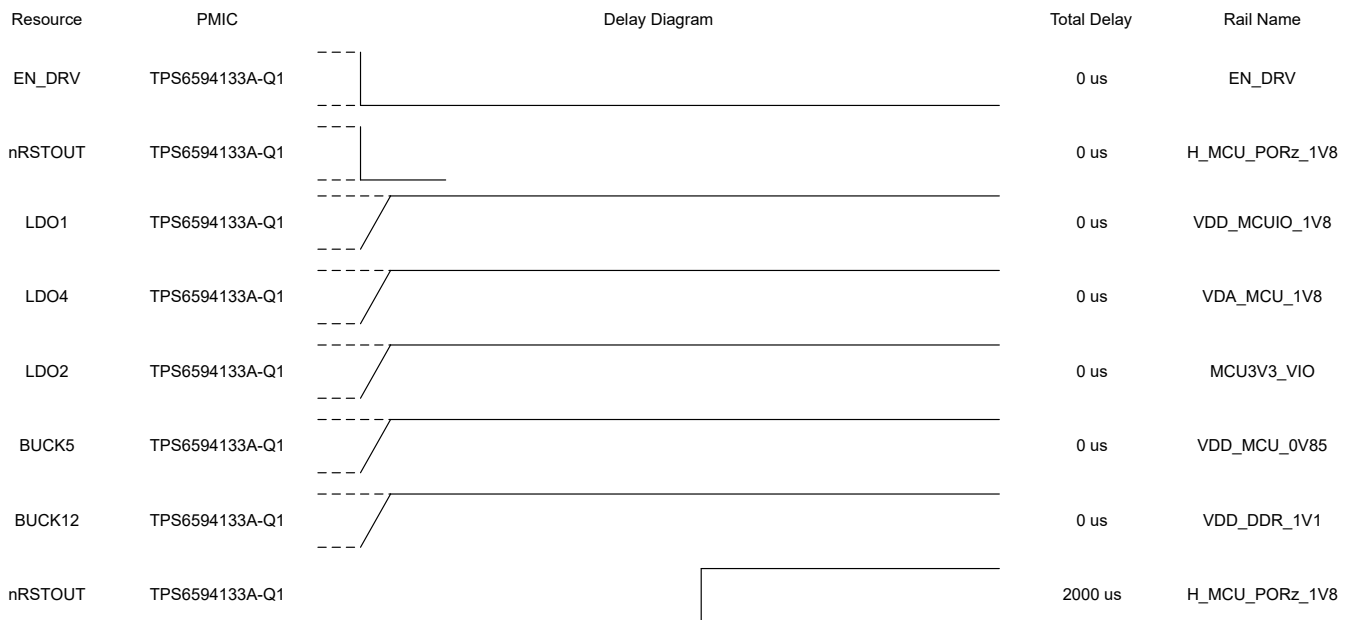
Figure 5-8. MCU_TO_WARM Sequence
