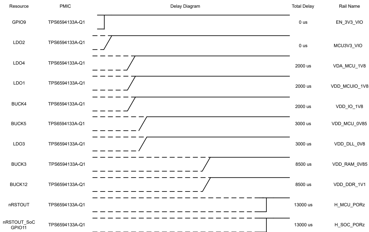
Figure 5-11. TO_ACTIVE Sequence
