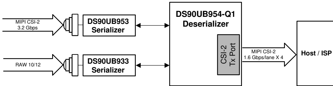
Figure 3-1. Applications Diagram
