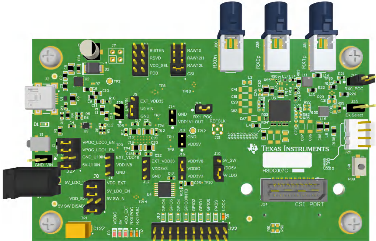
Figure 2-1. DS90UB954-Q1EVM
