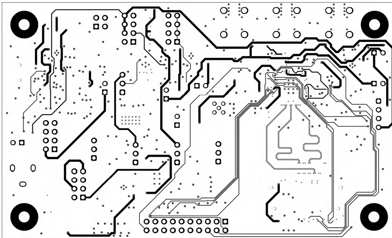
Figure 16-7. Layer 6: Mid Signal Layer 2
