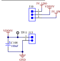
Figure 15-5. DS90UB954-Q1EVM Power Distribution Circuits - Page 4
