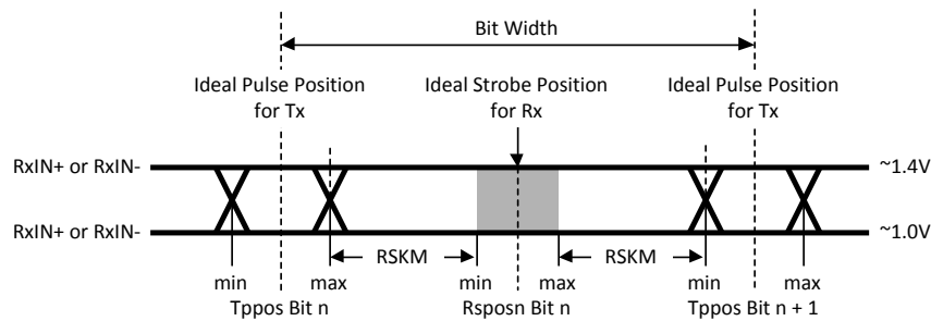
Figure 3. DS90CR218A (Receiver) Skew Margin
