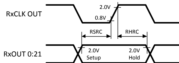
Figure 2. DS90CR218A (Receiver) Setup and Hold Time
