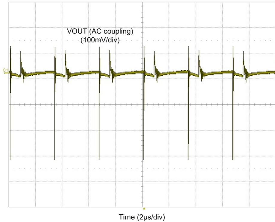
Figure 3. Output Voltage Ripple ( V_{IN} = 36\text{ V} , I_{OUT} = 2\text{ A} )
