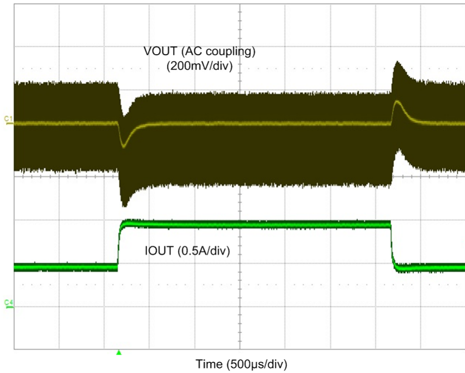
Figure 4. Load Transient Response ( V_{IN} = 36\text{ V} )
