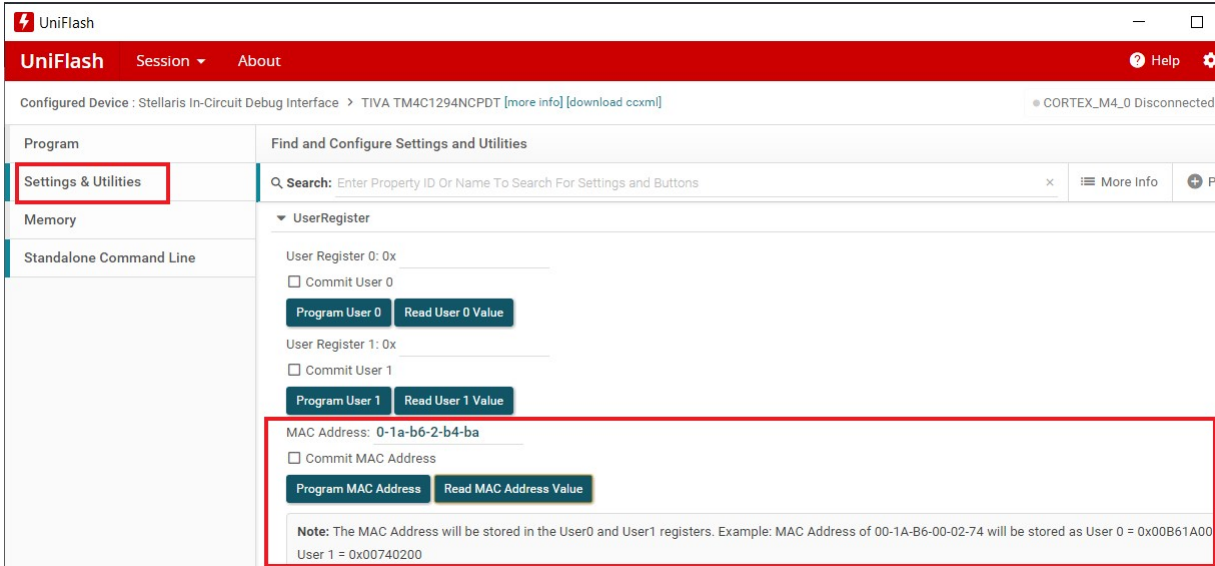
Figure 6-4. MAC Address Programming Using Uniflash
