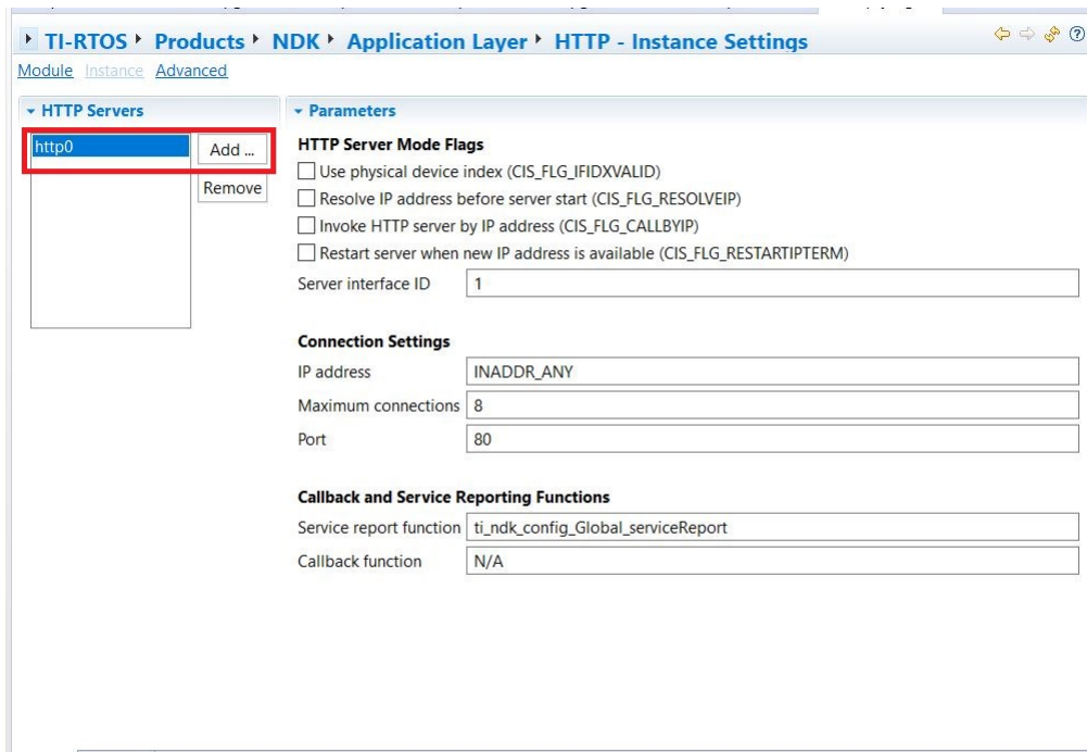
Figure 8-2. Adding a HTTP Instance
