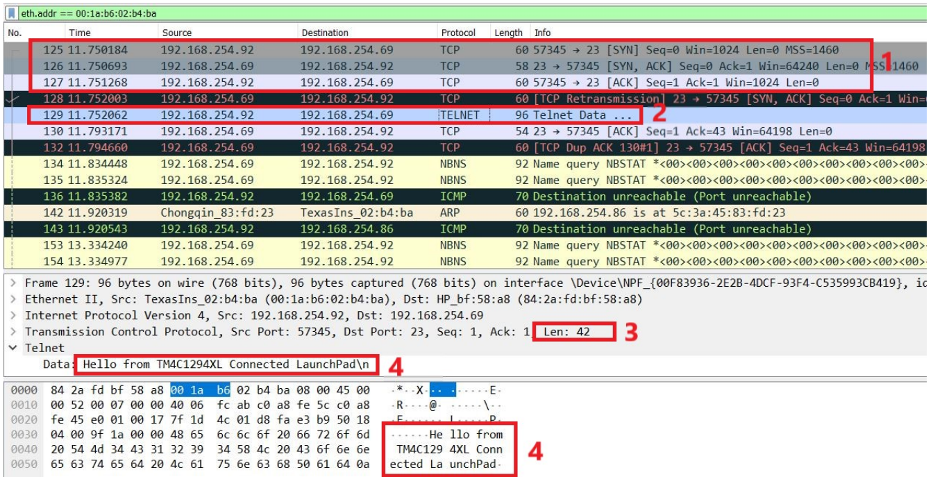
Figure 11-2. Client Server Wireshark Capture for Enet_tcpecho_client_tirtos
