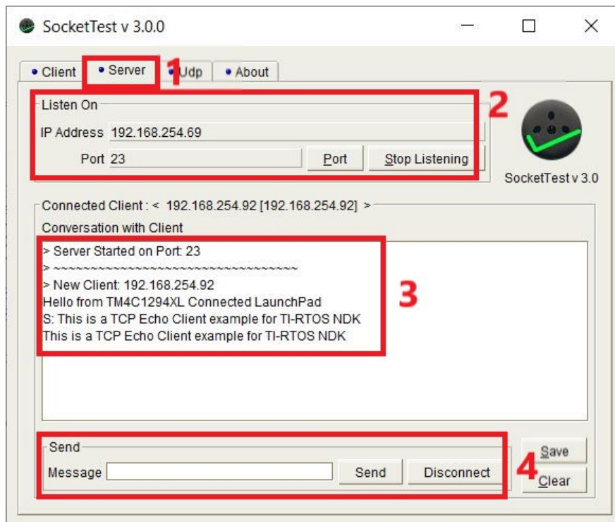
Figure 11-1. SocketTest Server Configuration for Enet_tcpecho_client_tirtos
