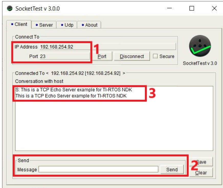
Figure 6-6. SocketTest Client Configuration for Enet_tcpecho_server_tirtos
