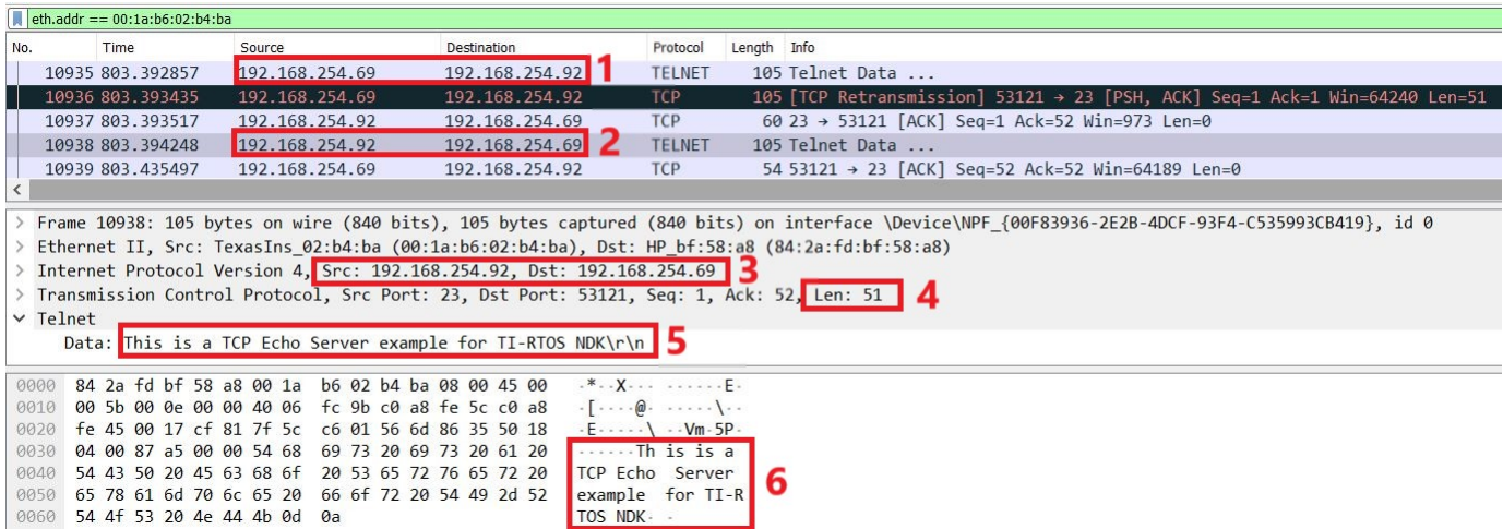
Figure 6-7. Server to Client Wireshark Capture for Enet_tcpecho_server_tirtos
