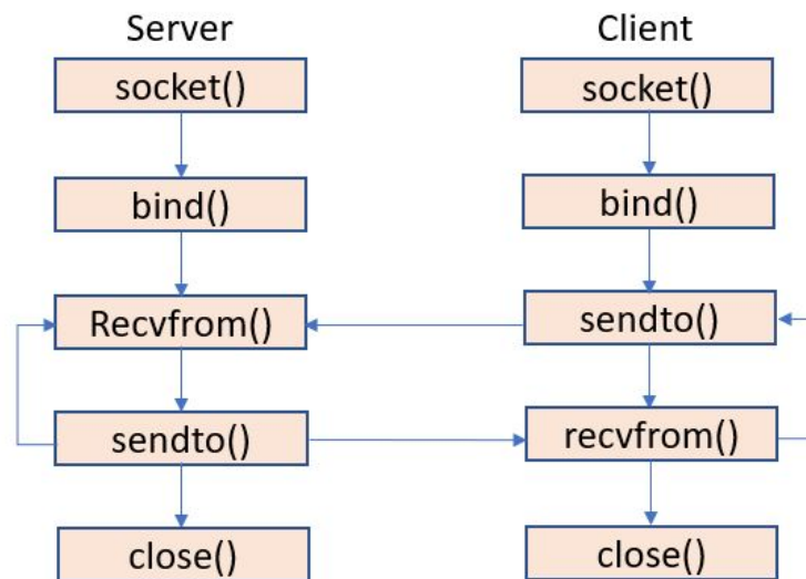
Figure 1-4. UDP Client Server Communication using BSD Socket APIs
