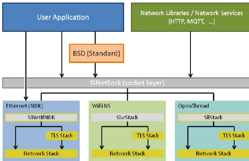
Figure 1-1. Components of a NDK-Enabled Application
