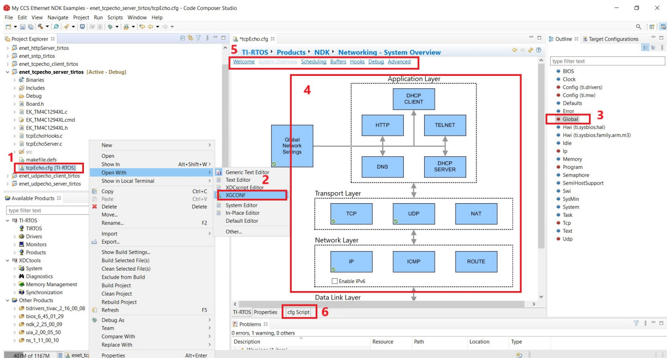
Figure 5-1. NDK Configuration Using XGCONF
