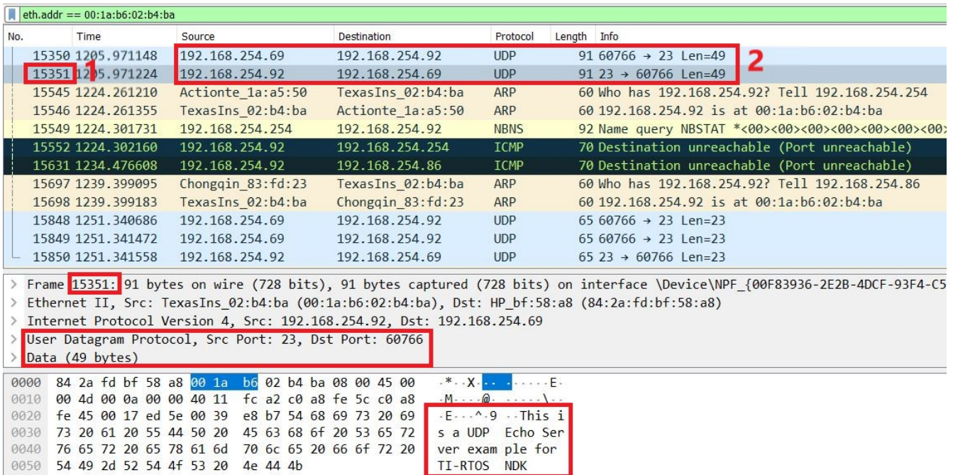
Figure 7-2. Server to Client Wireshark Capture for Enet_udpecho_server_tirtos
