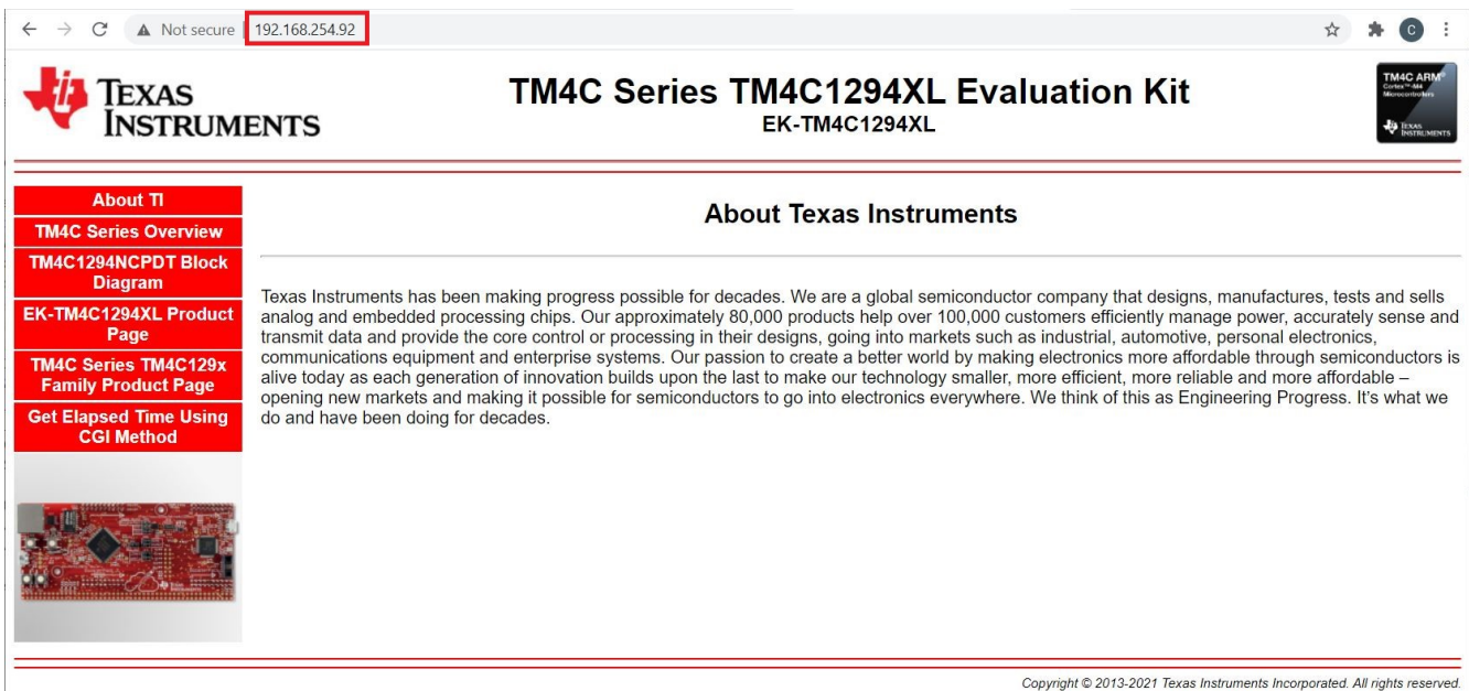
Figure 8-7. Enet_httpServer_tirtos Web Server Home Page
