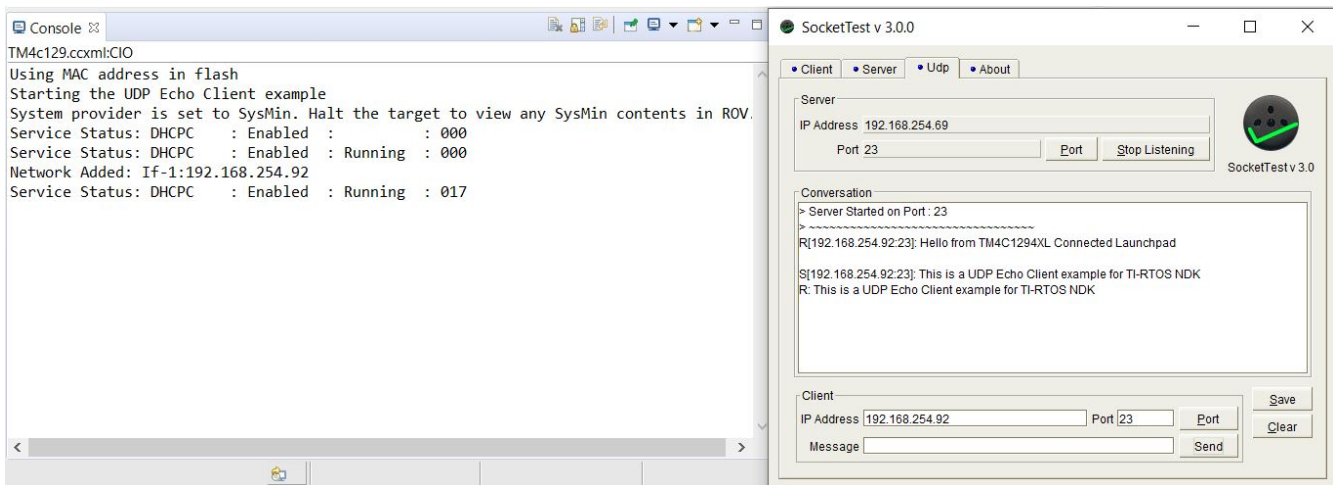
Figure 12-1. Enet_udpecho_client_tirtos Output
