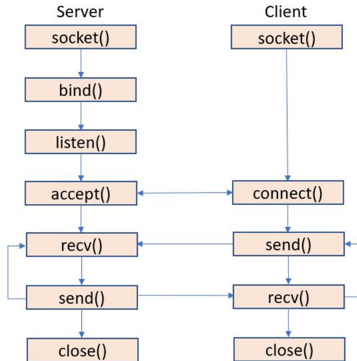
Figure 1-3. TCP Client Server Communication using BSD Socket APIs
