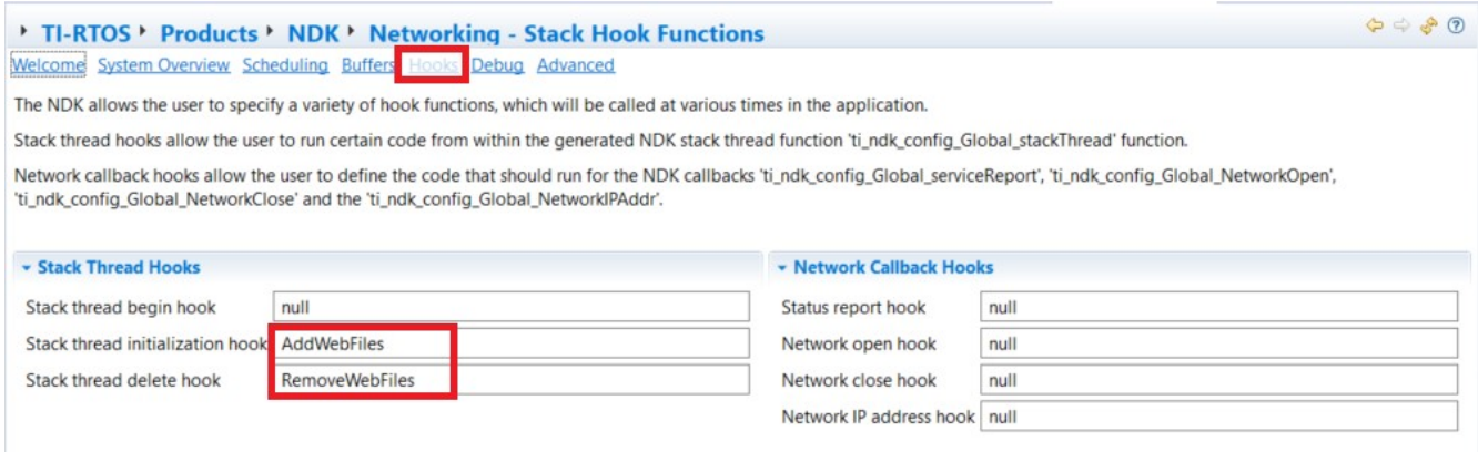
Figure 8-6. HTTP Hooks Declaration
