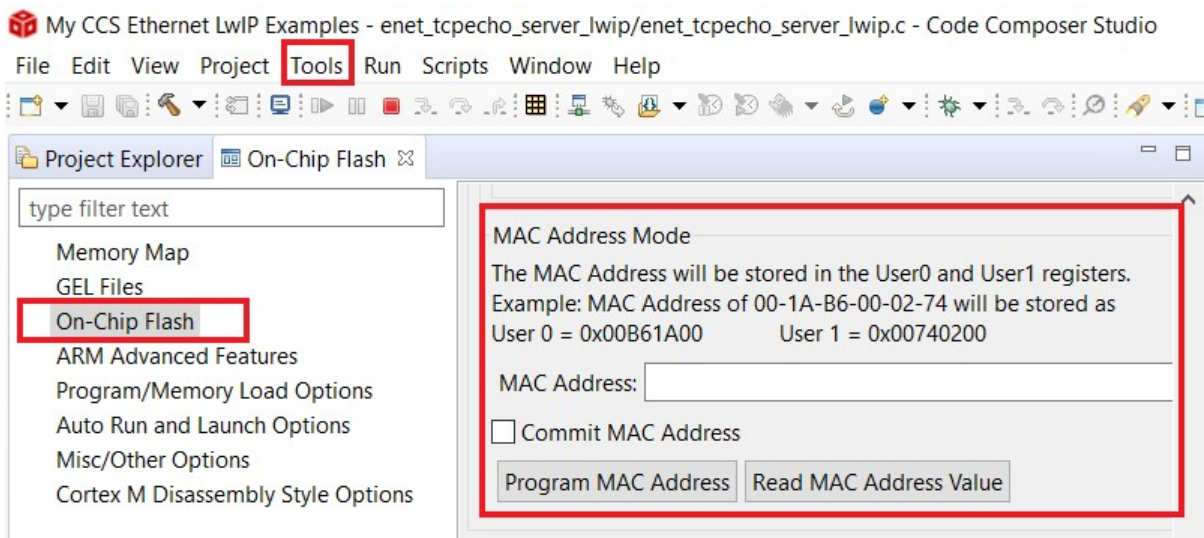
Figure 6-3. MAC Address Programming Using CCS
