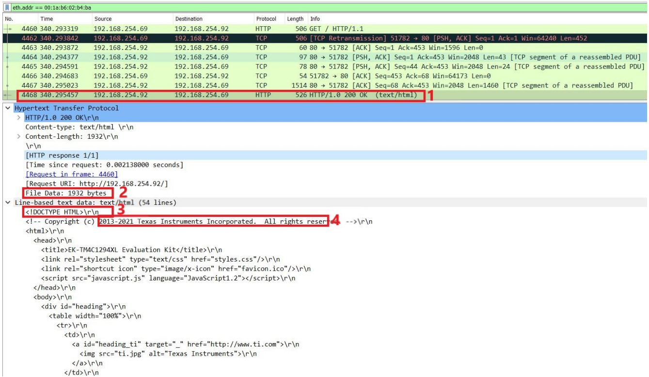
Figure 8-9. Wireshark Capture for enet_httpServer_tirtos Web Server
