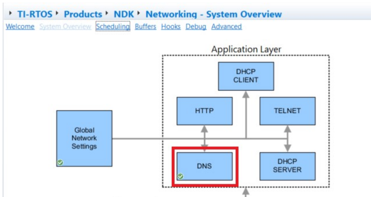
Figure 9-1. Configure NDK for DNS
