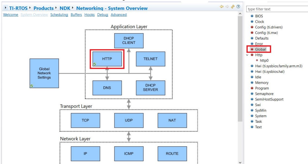
Figure 8-1. NDK Configuration for HTTP Application
