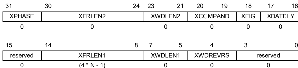
Figure 6. Transmit Control Register (XCR)
