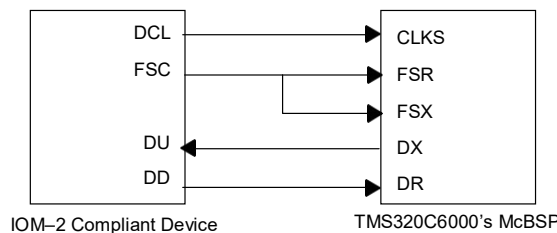
Figure 2. Connection Between the McBSP and an IOM-2 Compliant Device
