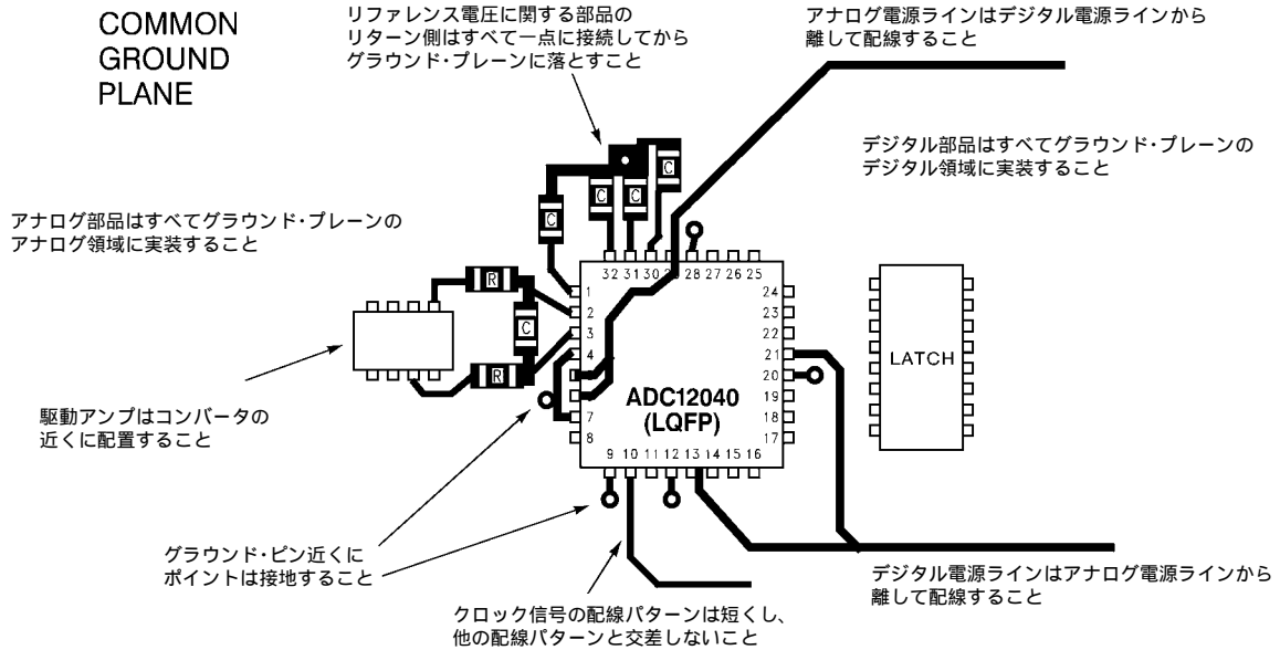
FIGURE 7. Example of a Suitable Layout
