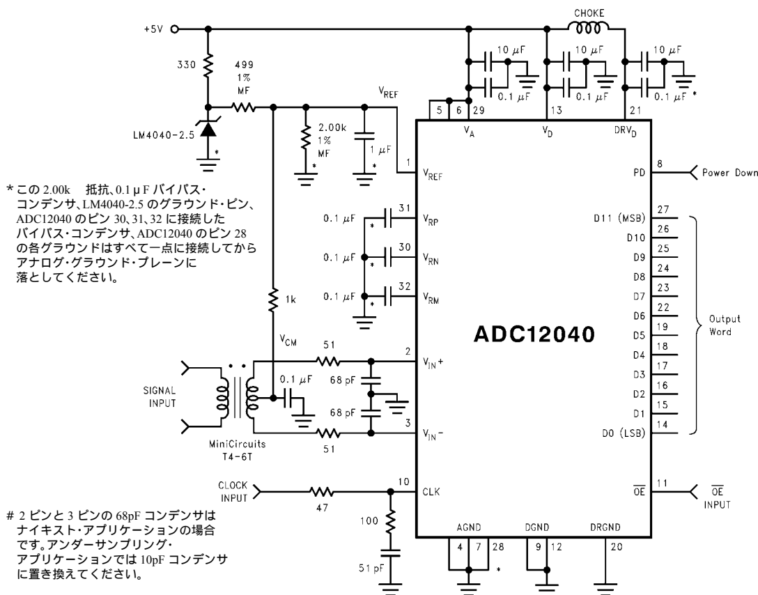
FIGURE 6. Driving the Signal Inputs with a Transformer
