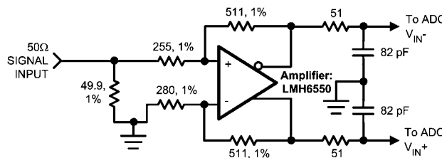
FIGURE 5. Differential Drive Circuit of Figure 4
