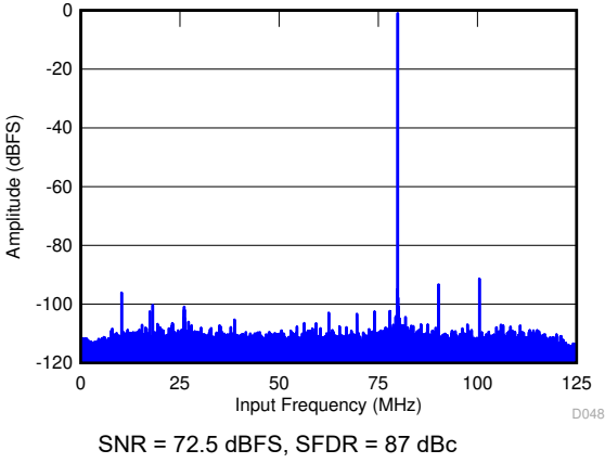
7-51. FFT for 170-MHz Input Signal in Decimate-by-4 Mode
