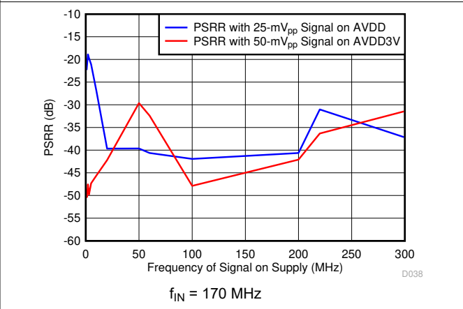
7-44. Power-Supply Rejection Ratio vs Test Signal Frequency
