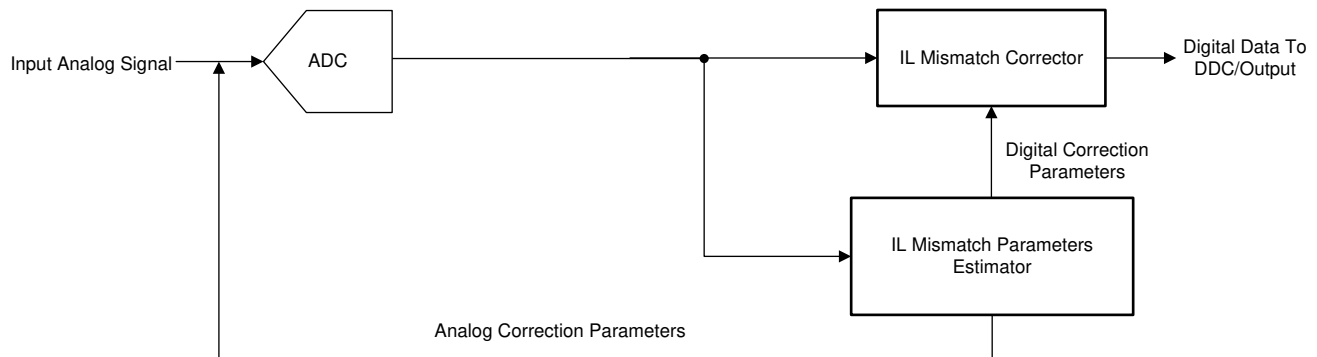
9-9. Block diagram of Interleaving mismatch Compensation
