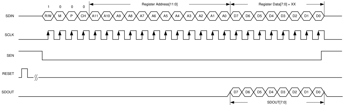
Figure 8-14. Serial Register Read Timing Diagram
