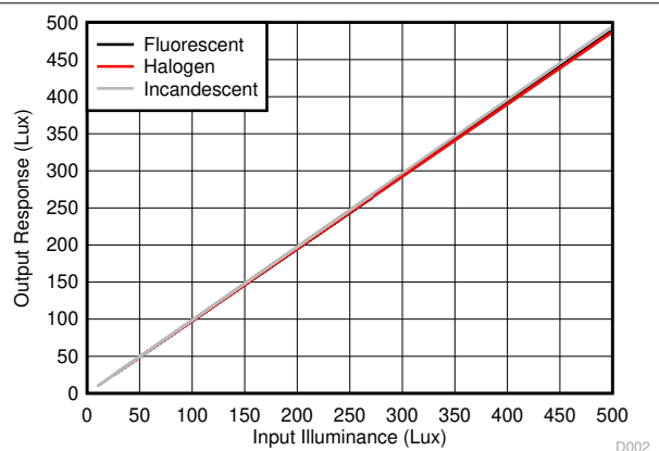
5-3. Output Response vs Input Illuminance, Multiple Light Sources: Fluorescent, Halogen, Incandescent
