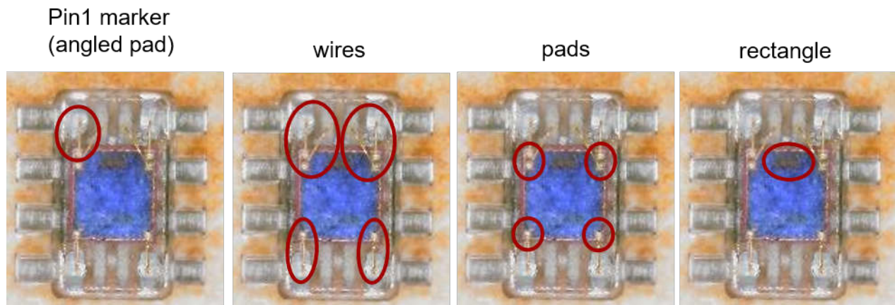
☒ 11-4. Identifying DTS Package Orientation - Backside
