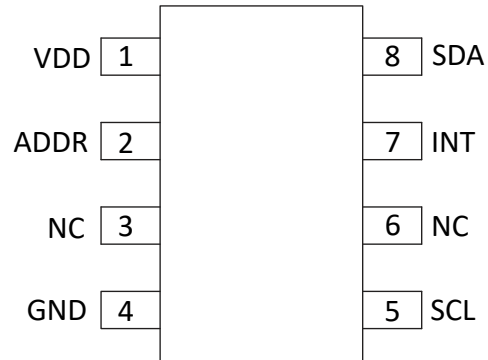
図 4-2. DTS Package 8-Pin SOT-5X3 Top View
