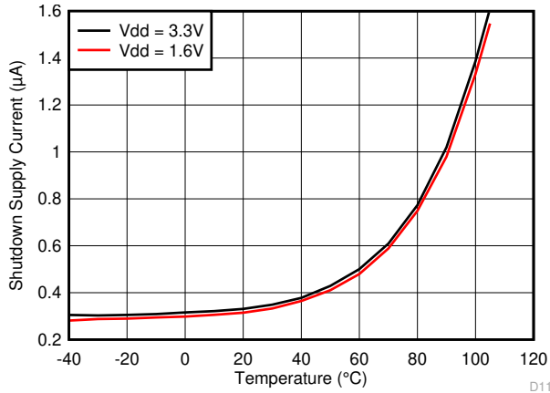
5-20. Shutdown Current vs Temperature (Grade 2)
