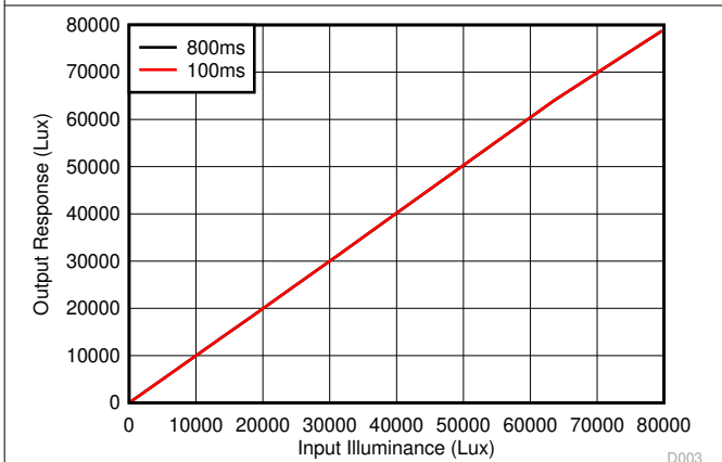
5-4. Output Response vs Input Illuminance: Entire Range = 0lux to 83klux
