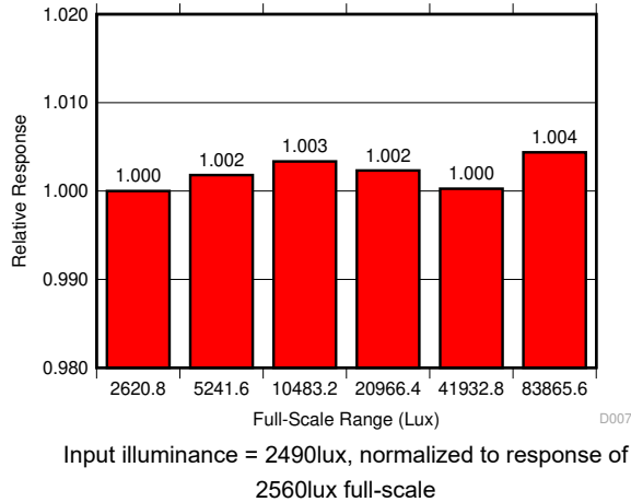
5-8. Full-Scale-Range Matching (Highest 6 Ranges)
