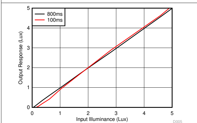
5-6. Output Response vs Input Illuminance: Low Range = 0lux to 5lux
