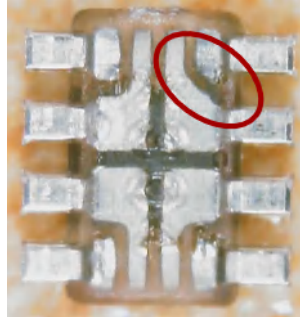
☒ 11-4. Identifying DTS Package Orientation - Backside
