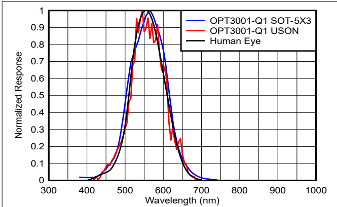
5-2. Spectral Response vs Wavelength
