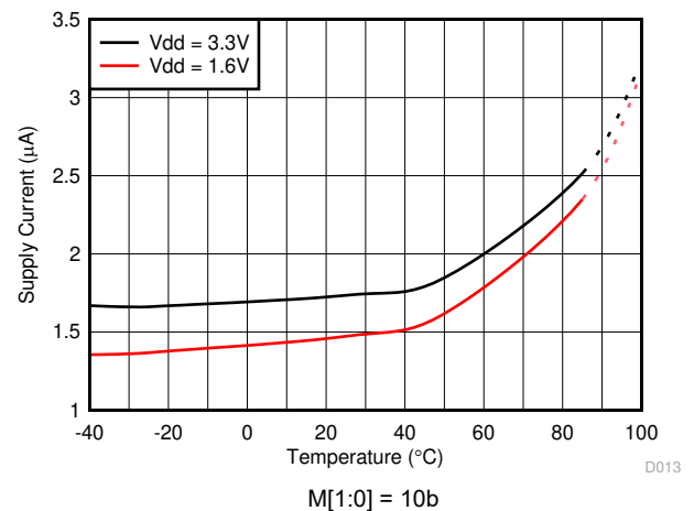
5-19. Supply Current vs Temperature (Grade 3)
