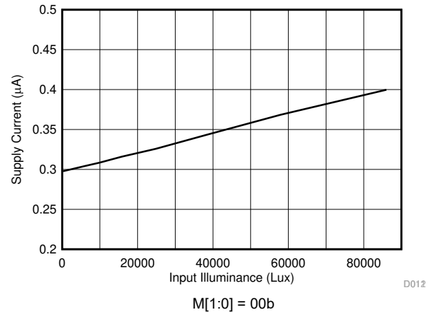
5-17. Shutdown Current vs Input Illuminance
