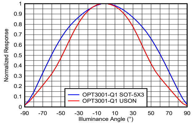
5-15. Normalized Response vs Illuminance Angle
