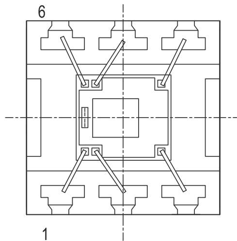
☒ 11-1. Package Orientation Visual Reference of Pin 1 (Top View)
