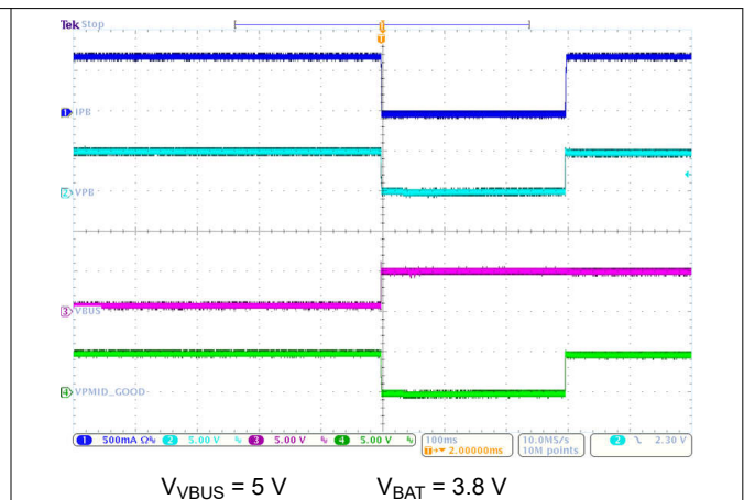
8-3. VBUS Plugged In with Boost Mode Enabled
