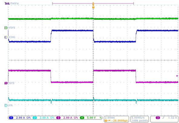
図 8-7. System Load Transient Response
