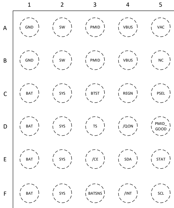
5-1. BQ25618 YFF Package 30-Pin WCSP Top View
