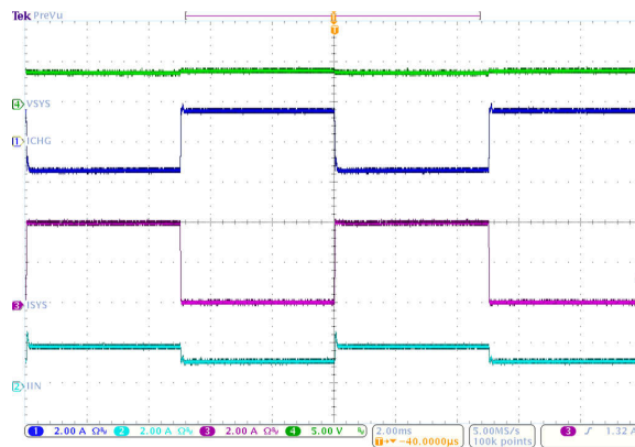
図 8-8. System Load Transient Response
