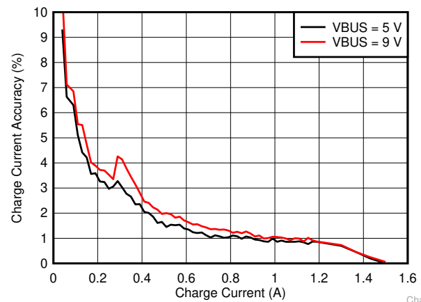
6-5. Charge Current Accuracy
