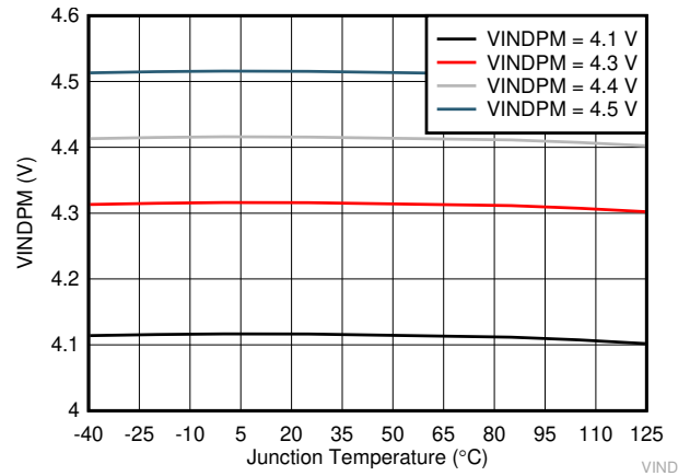
6-8. VINDPM vs Junction Temperature
