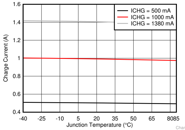
6-7. Charge Current vs Junction Temperature
