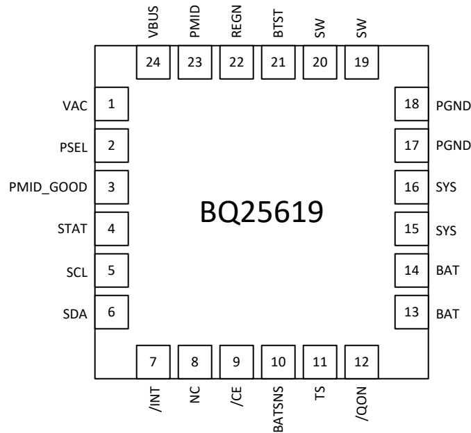
5-2. BQ25619 RTW Package 24-Pin WQFN Top View
