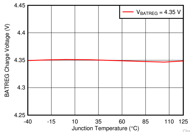
6-6. Battery Charge Voltage vs Junction Temperature
