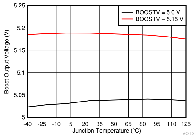
6-11. Boost Output Voltage vs Junction Temperature
