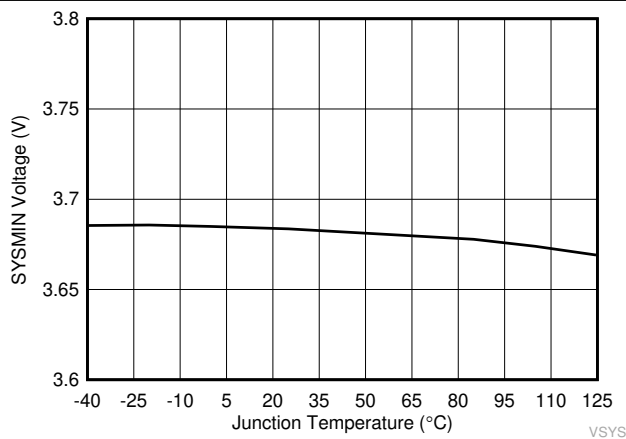
6-9. SYSMIN Voltage vs Junction Temperature (VSYS set at 3.5 V)
