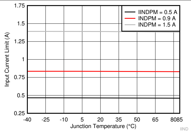
6-10. Input Current Limit vs Junction Temperature
