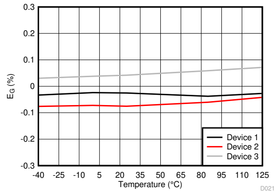
6-18. Gain Error vs Temperature
