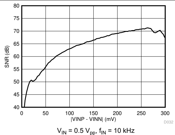
6-22. Signal-to-Noise Ratio vs Input Voltage
