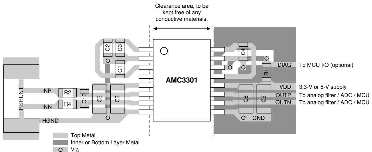
☒ 10-1. Recommended Layout of the AMC3301
