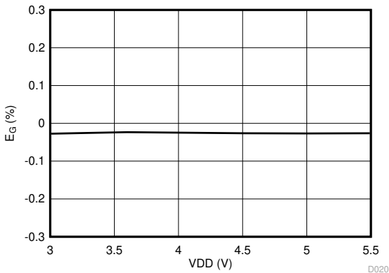
6-17. Gain Error vs Supply Voltage
