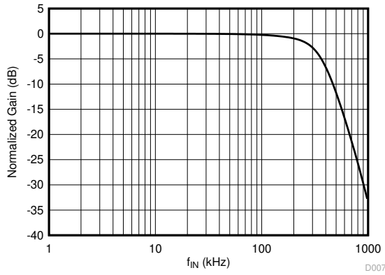
6-11. Normalized Gain vs Input Frequency
