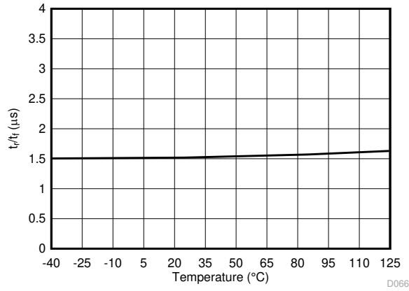
6-35. Output Rise and Fall Time vs Temperature
