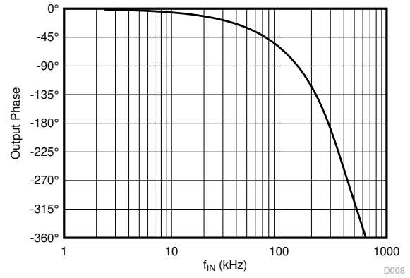
6-12. Output Phase vs Input Frequency
