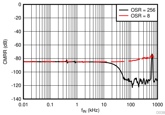
6-36. Common-Mode Rejection Ratio vs Input Signal Frequency
