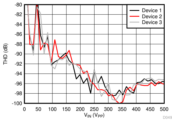
6-24. Total Harmonic Distortion vs Input Signal Amplitude
