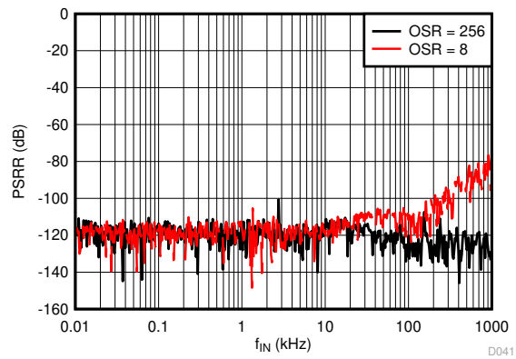
6-37. Power-Supply Rejection Ratio vs Ripple Frequency
