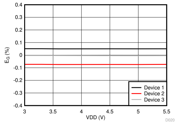
6-13. Gain Error vs Supply Voltage
