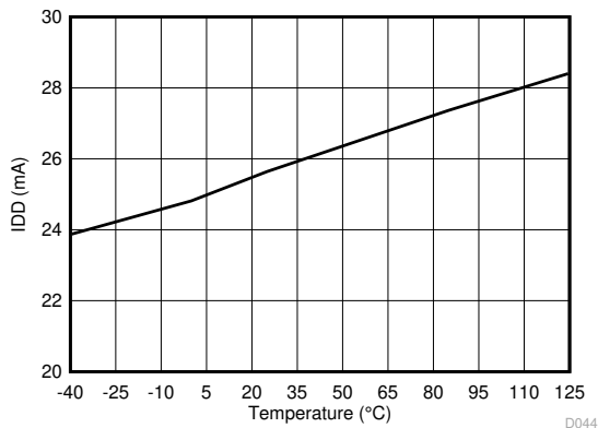
6-40. Supply Current vs Temperature
