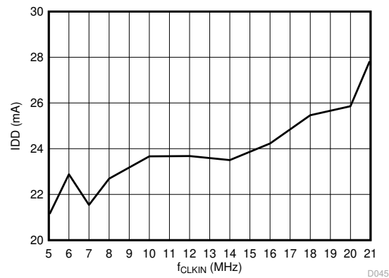
6-39. Supply Current vs Input Clock Frequency
