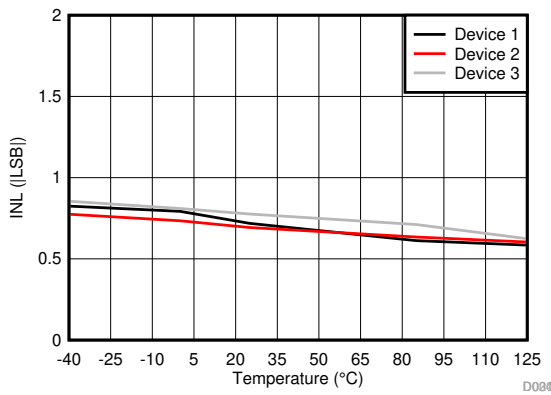
6-18. Integral Nonlinearity vs Temperature
