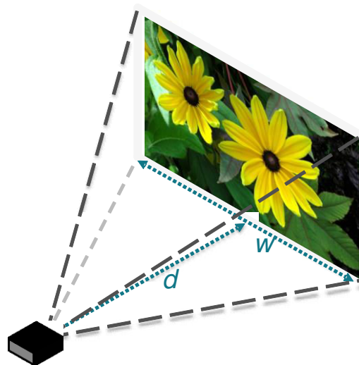
Figure 2-3. Throw Ratio
