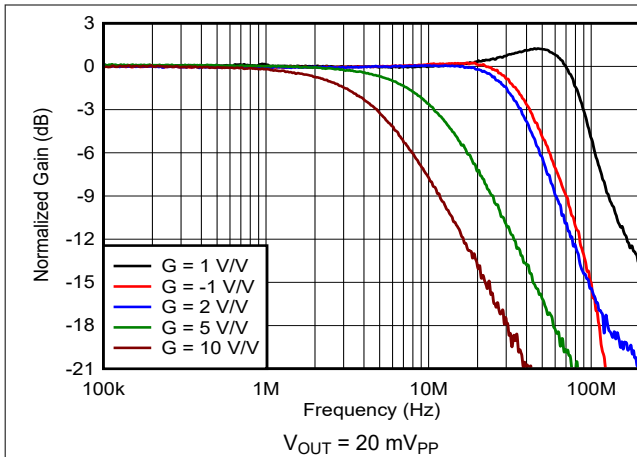
Figure 6-28. Small-Signal Frequency Response vs Gain
