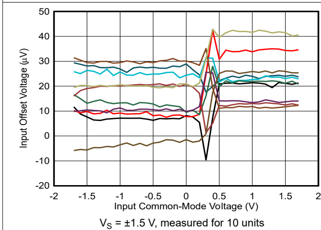
Figure 6-32. Input Offset Voltage vs Input Common-Mode Voltage
