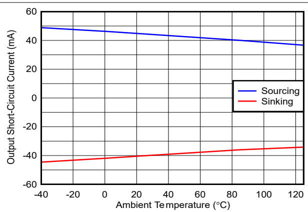
Figure 6-35. Output Short-Circuit Current vs Ambient Temperature Output saturated and then short-circuited to other supply
