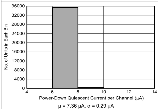
Figure 6-38. Power-Down Quiescent Current Distribution \mu = 7.36\ \mu\text{A} , \sigma = 0.29\ \mu\text{A}
