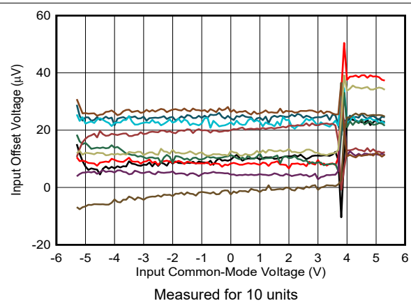
Figure 6-12. Input Offset Voltage vs Input Common-Mode Voltage Measured for 10 units
