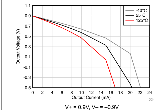
Figure 5-23. Output Voltage Swing vs Output Current (Sourcing)
