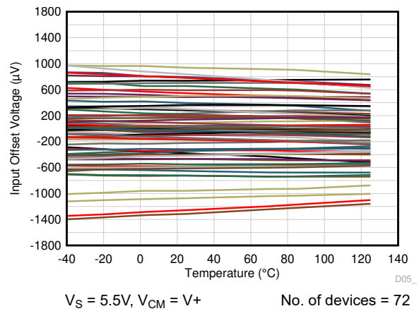
Figure 5-8. Input Offset Voltage vs Temperature
