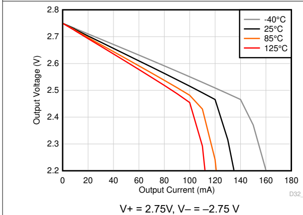
Figure 5-21. Output Voltage Swing vs Output Current (Sourcing)
