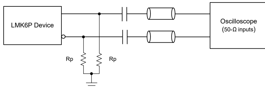
Figure 7-5. LMK6P Output Test Configuration
