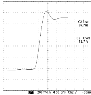
Figure 59. Rise Time
