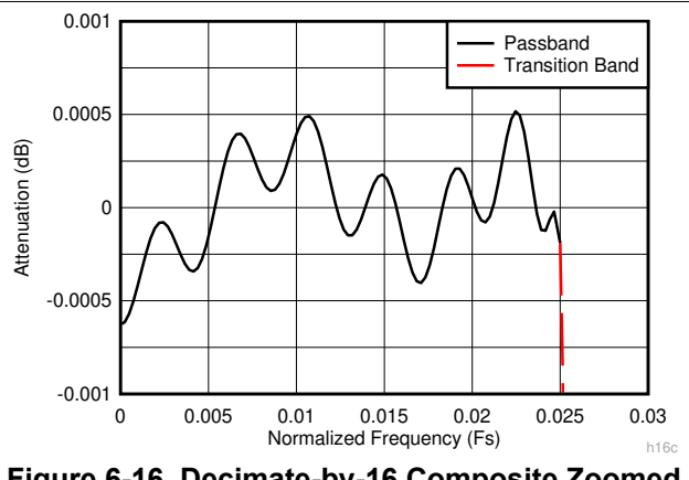
Figure 6-16. Decimate-by-16 Composite Zoomed Pass-Band Response
