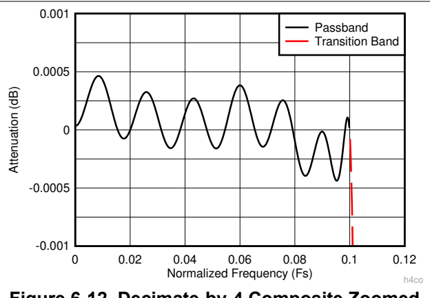
Figure 6-12. Decimate-by-4 Composite Zoomed Pass-Band Response
