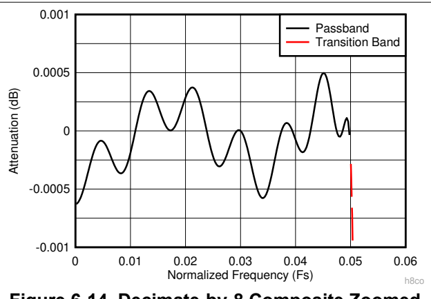
Figure 6-14. Decimate-by-8 Composite Zoomed Pass-Band Response
