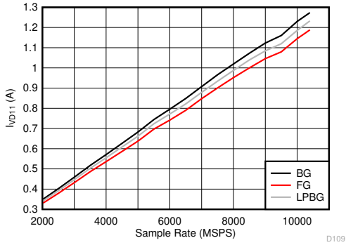
Figure 6-127. DES Mode: I_{VD11} vs Sample Rate
