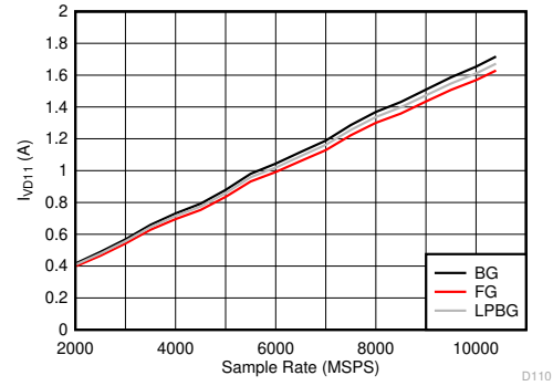
Figure 6-128. DES Mode: I_{VD11} vs Sample Rate
