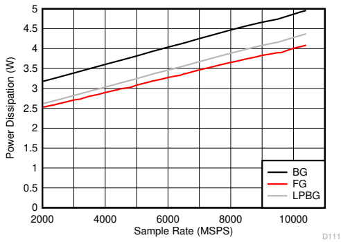
Figure 6-129. DES Mode: Power Dissipation vs Sample Rate
