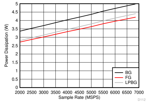
Figure 6-130. DES Mode: Power Dissipation vs Sample Rate
