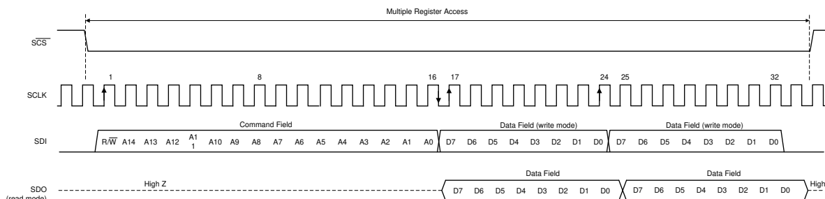
Figure 7-27. Serial Interface Protocol: Streaming Read/Write
