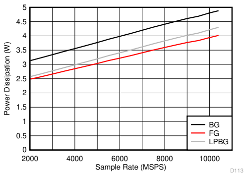
Figure 6-131. DES Mode: Power Dissipation vs Sample Rate
