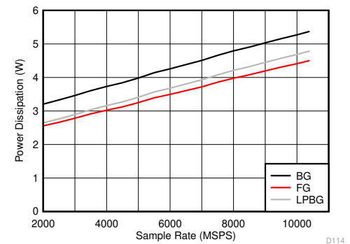
Figure 6-132. DES Mode: Power Dissipation vs Sample Rate
