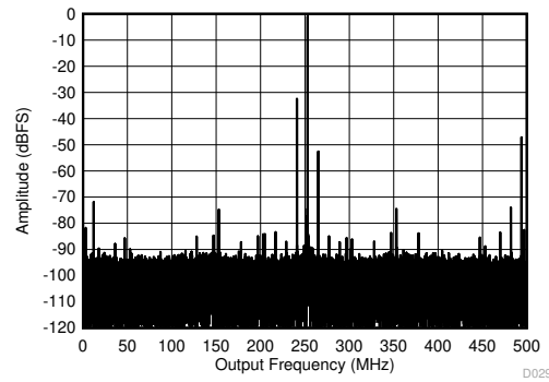
Low power mode, F_S = 1000 MSPS Figure 8-16. Single Tone FFT at 3797 MHz and -1 dBFS
