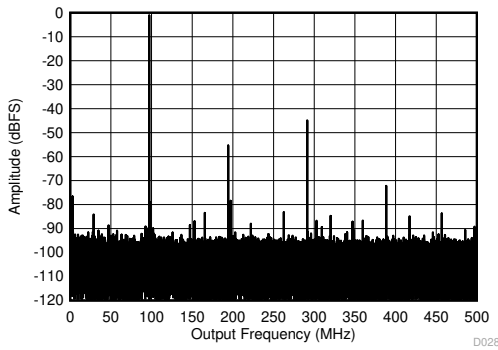
Low power mode, F_S = 1000 MSPS Figure 8-15. Single Tone FFT at 2097 MHz and -1 dBFS
