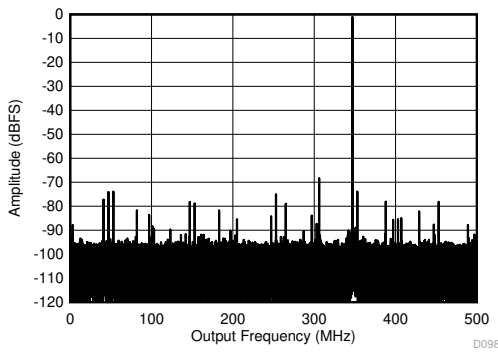
C-PLL on, Low power mode, F_S = 1000 MSPS Figure 8-13. Single Tone FFT at 347 MHz and -1 dBFS
