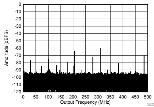
Low power mode, F_S = 1000 MSPS Figure 8-14. Single Tone FFT at 897 MHz and -1 dBFS
