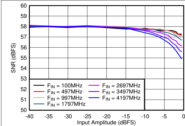
Figure 8-33. SNR vs A_{IN}
