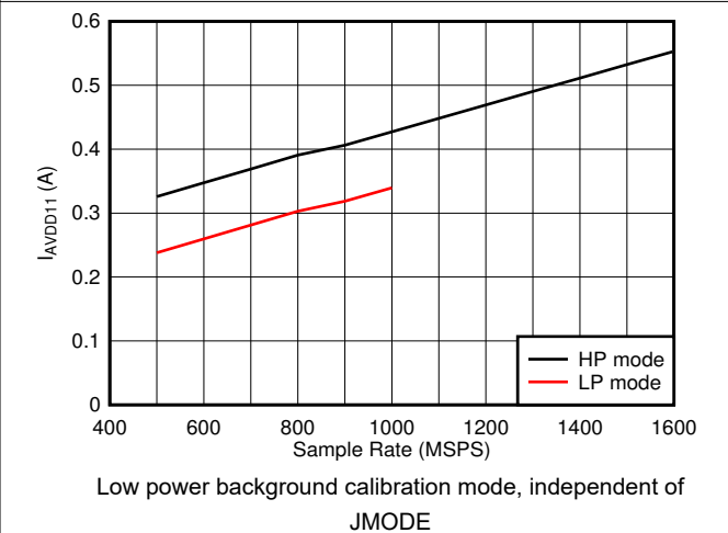
Figure 7-94. Dual Channel, I_{VA11} vs F_S
