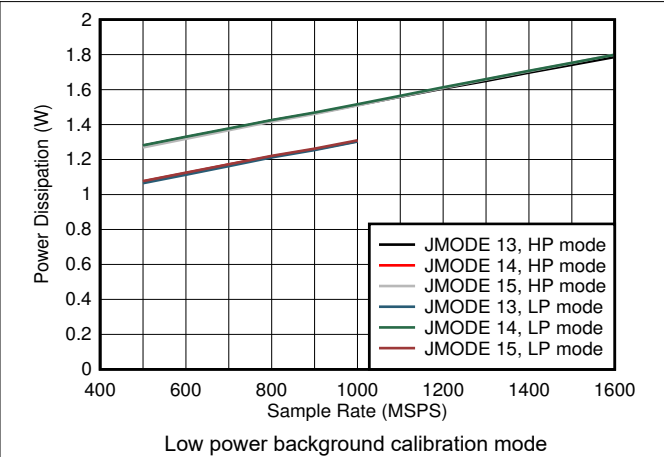
Figure 7-92. Dual Channel, Power Dissipation vs F_S and JMODE 13 - 15
