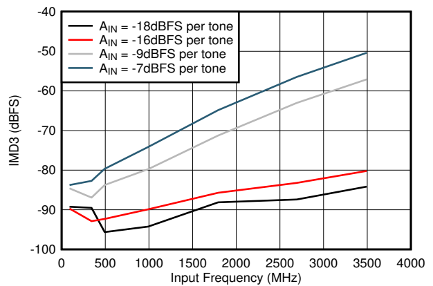
10MHz tone spacing, Low power mode, 1000MSPS Figure 7-76. IMD3 vs F_{IN}
