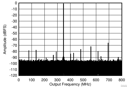
High power mode Figure 7-4. Single Tone FFT at 347 MHz and -1 dBFS
