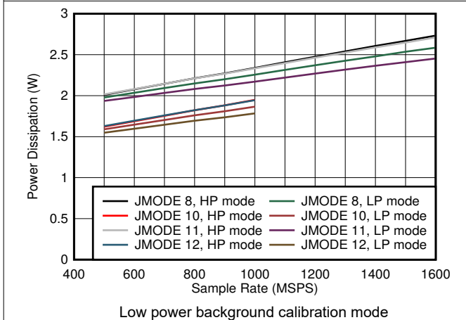
Figure 7-81. Quad Channel, Power Dissipation vs F_S and JMODE 8 - 12
