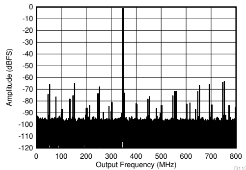
High power mode, C-PLL on, Noise suppression off Figure 7-6. Single Tone FFT at 347 MHz and -1 dBFS
