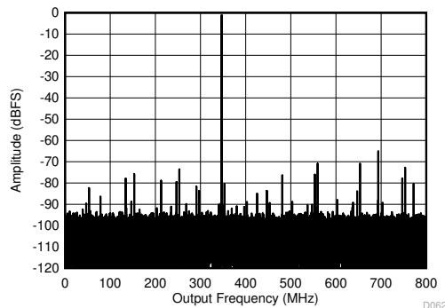
High power mode, C-PLL on Figure 7-5. Single Tone FFT at 347 MHz and -1 dBFS
