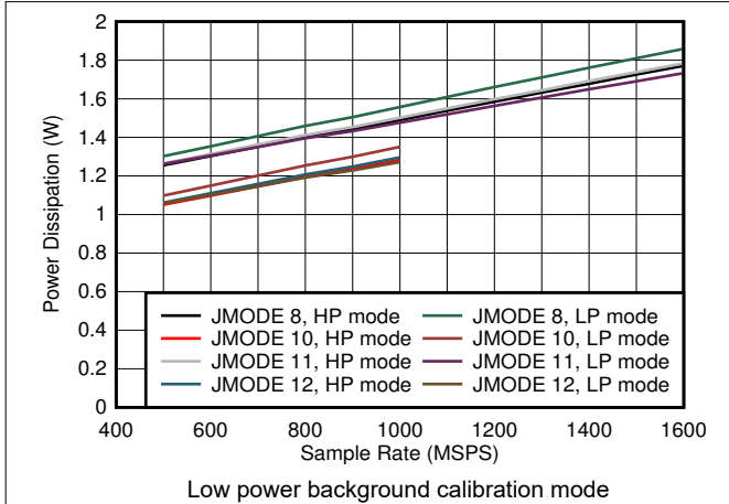
Figure 7-91. Dual Channel, Power Dissipation vs F_S and JMODE 8 - 12
