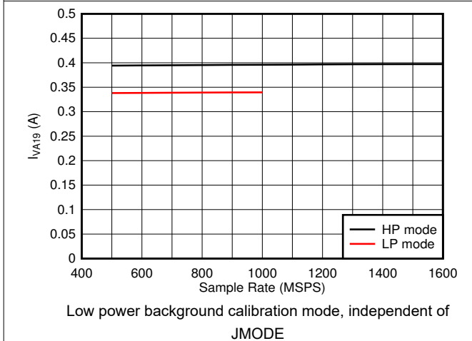
Figure 7-93. Dual Channel, I_{VA19} vs F_S
