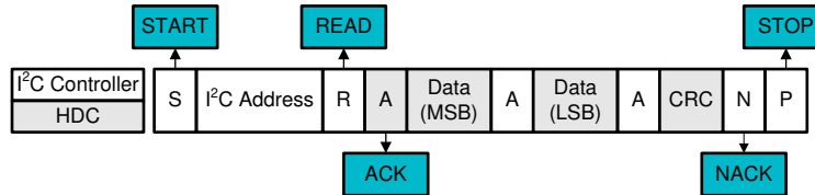
Figure 8-6. I 2 C Read Single Data Result, CRC Retained
