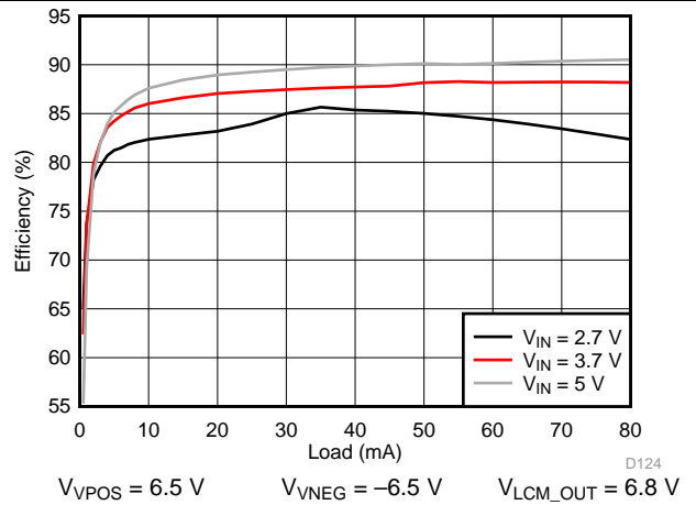
Figure 174. VPOS/VNEG Efficiency
