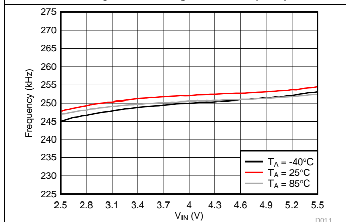
Figure 10. Backlight Boost Frequency
