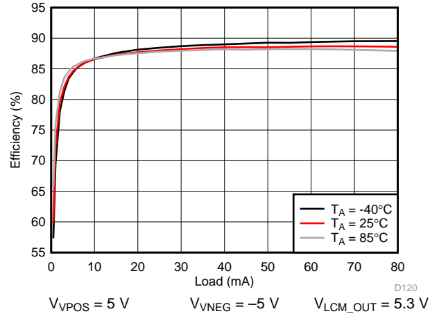
Figure 170. VPOS/VNEG Efficiency
