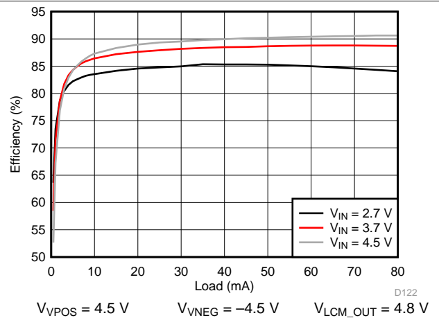
Figure 172. VPOS/VNEG Efficiency
