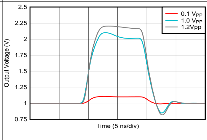
Figure 5-10. Pulse Response vs Output Swing
