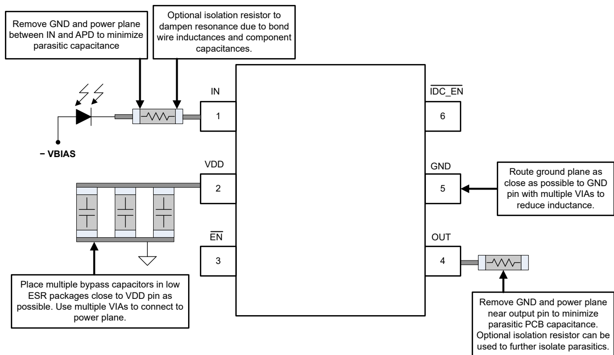
Figure 7-10. Layout Recommendation
