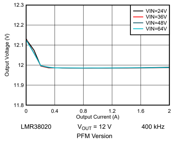
LMR38020 V_{OUT} = 12\text{ V} 400 kHz PFM Version
