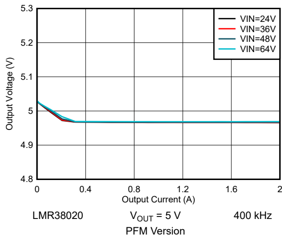
LMR38020 V_{OUT} = 5\text{ V} 400 kHz PFM Version
