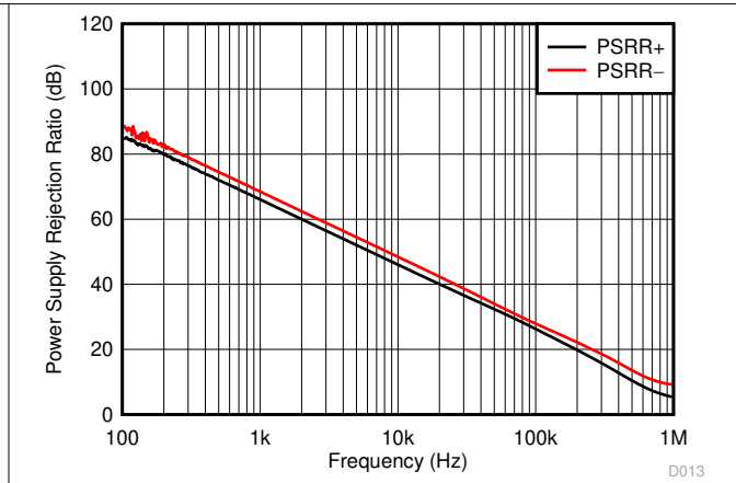
Figure 6-8. PSRR vs Frequency
