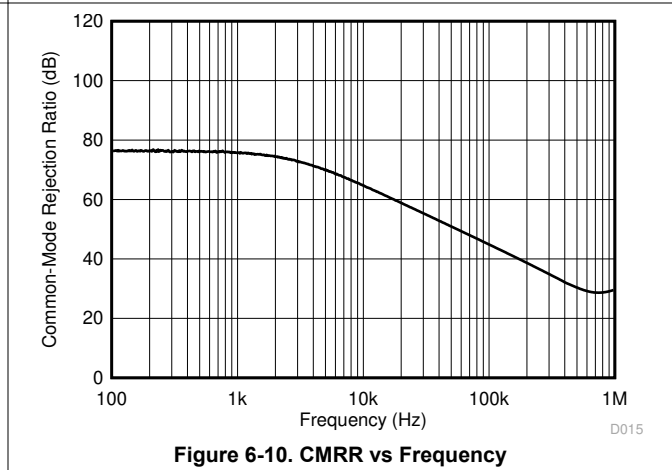
Figure 6-10. CMRR vs Frequency
