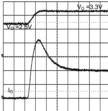
Figure 35. Prebiased Start-Up
