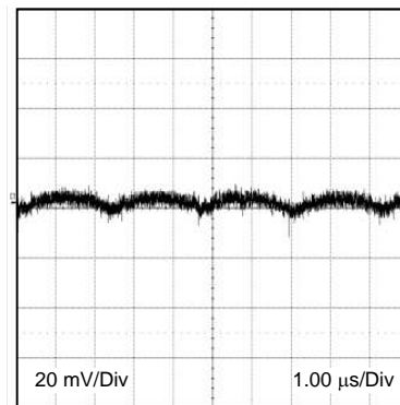
12 V_{IN} 3.3 V_O 2 A 20 mV/div 1 μs/div
