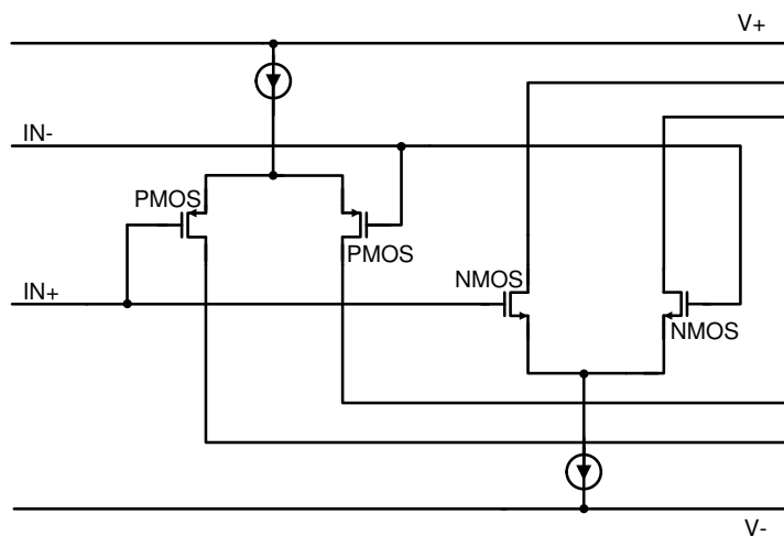
Figure 6-8. Rail-to-Rail Input Stage
