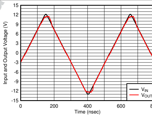
Figure 6-27. Large-Signal Transient Response
