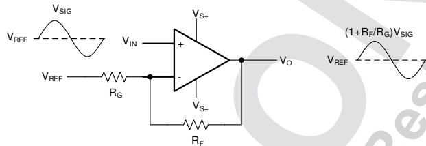
Figure 8-1. Noninverting Amplifier
