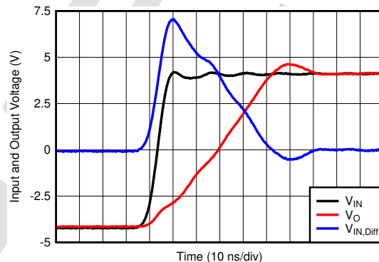
Figure 8-18. Large-Signal Transient Response Using the OPA810
