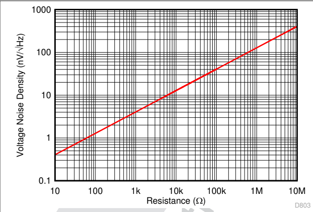
Figure 8-9. Thermal Noise Density vs. Resistance
