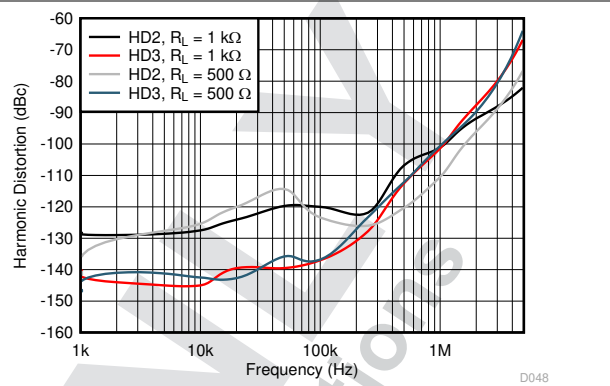
See Figure 8-1, gain = 2 V/V
