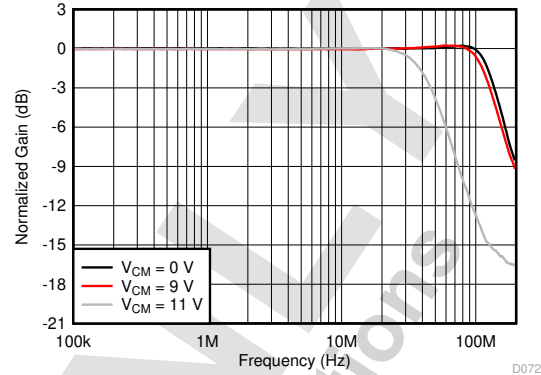
See Figure 8-1, V_O = 20\text{ mV}_{PP} , gain = 1 V/V, C_L = 4.7\text{ pF} , R_F = 0\ \Omega
