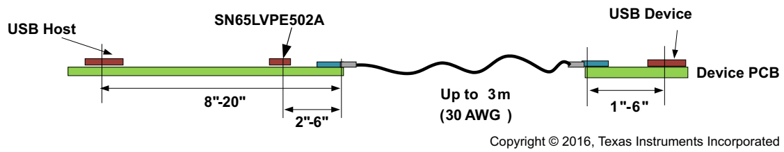
Figure 6. Redriver Placement Example
