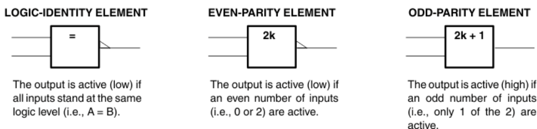
Figure 7-1. Exclusive-OR Logic
