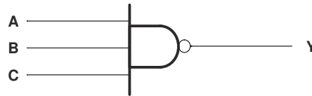
Figure 6-1. Logic Diagram, Each Gate (Positive Logic)
