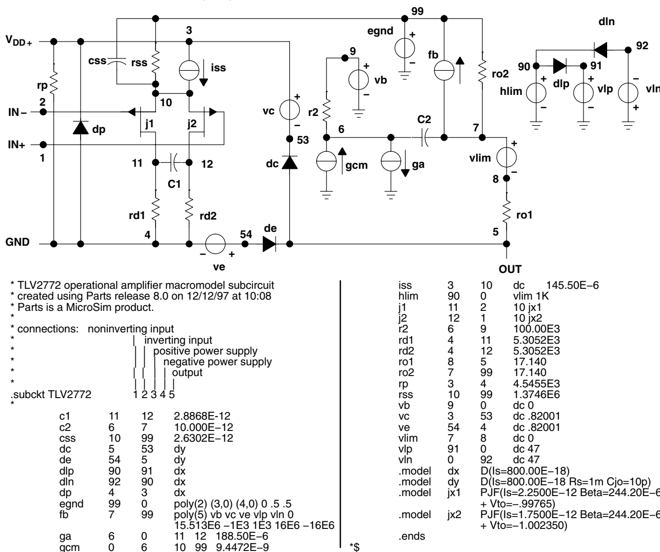
Figure 64. Boyle Macromodel and Subcircuit
