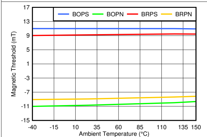
Figure 7-11. TMAG5123D Magnetic Thresholds vs. Temperature
