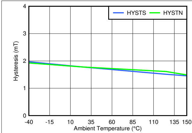
Figure 7-13. TMAG5123D Hysteresis vs. Temperature
