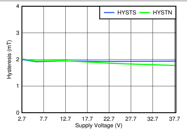
Figure 7-10. TMAG5123C Hysteresis vs. Supply Voltage
