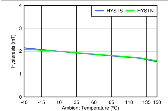
Figure 7-9. TMAG5123C Hysteresis vs. Temperature
