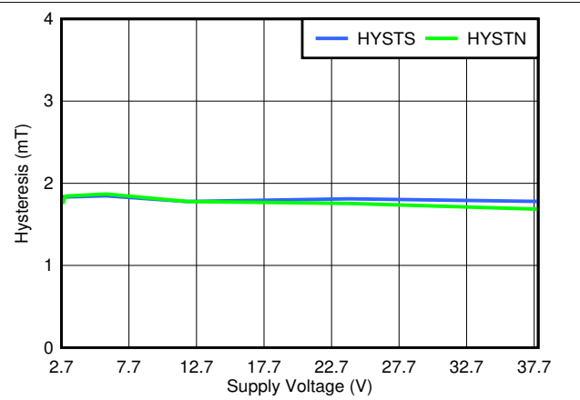
Figure 7-14. TMAG5123D Hysteresis vs. Supply Voltage
