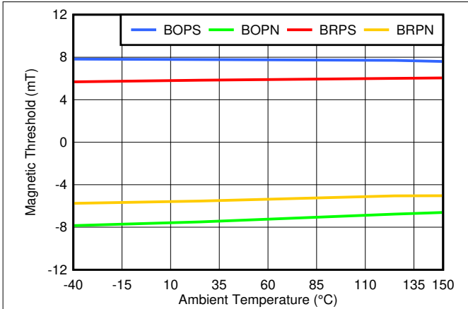
Figure 7-7. TMAG5123C Magnetic Thresholds vs. Temperature
