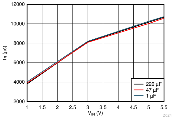
Figure 7-19. Turn-On vs Load Capacitance (CT = 10000 pF)
