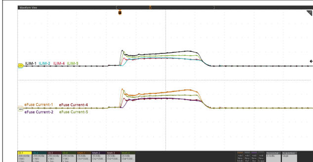
Figure 9-6. Start-up with EN/UVLO (Current distribution among five devices in parallel): V_{IN} = 12 V, EN/UVLO Stepped Up From 0 V to 3 V, C_{LOAD} = 55 mF, C_{DVDT} = 33 nF, R_{IREF} = 40.2 k \Omega , and R_{ILIM} on Each Device = 300 \Omega
