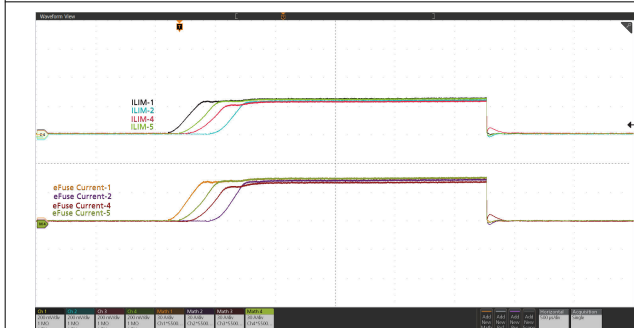
Figure 9-8. Power Up into Short (Current distribution among five devices in parallel): V_{IN} = 12 V, EN/UVLO Stepped Up From 0 V to 3 V, R_{IREF} = 40.2 k \Omega , R_{ILIM} on Each Device = 300 \Omega , and OUT Shorted to GND
