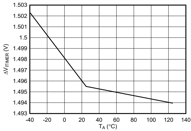
Figure 7-17. ITIMER Pin Discharge Differential Voltage Threshold Across Temperature
