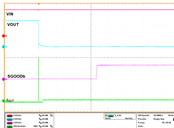
Figure 7-23. Fast-Trip Protection
